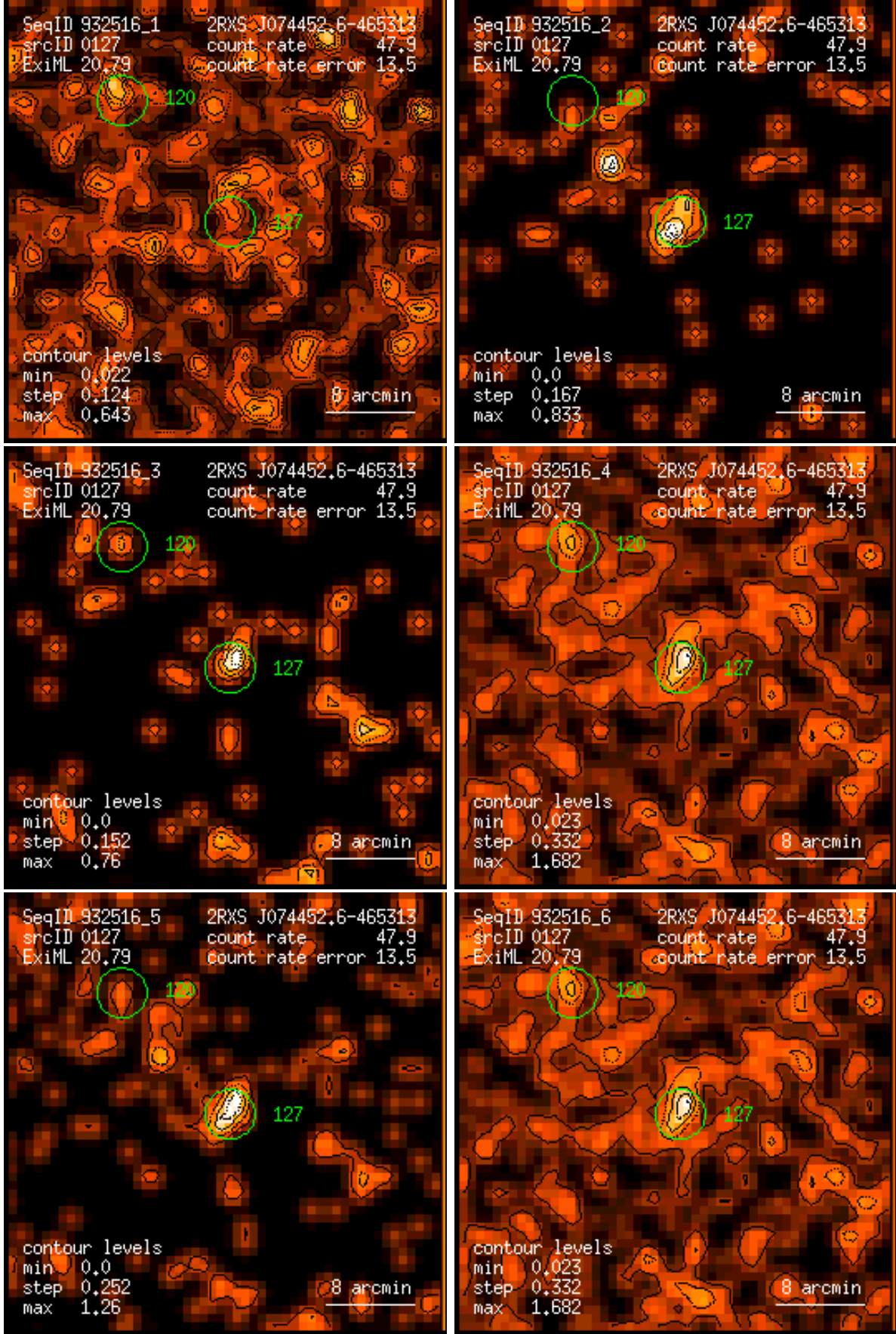
Figure 127: RASS 932516: detection 0127: band rate images, Gaussian filter: (1) PSPC channels 11 – 41, (2) 52 – 90, (3) 91 – 201, (4) 11 – 235, (5) 52 – 201, (6) 11 – 201. Broad band rates in counts/ks. Band rate contour levels in counts/ks/arcmin 2 .
