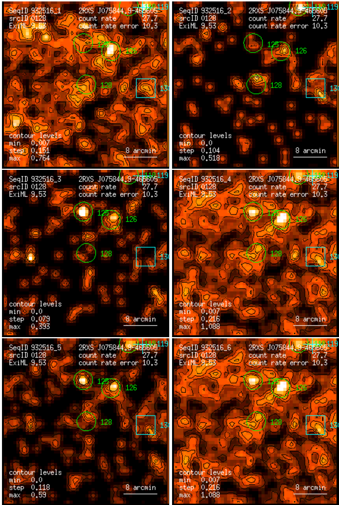
Figure 128: RASS 932516: detection 0128: band rate images, Gaussian filter: (1) PSPC channels 11 – 41, (2) 52 – 90, (3) 91 – 201, (4) 11 – 235, (5) 52 – 201, (6) 11 – 201. Broad band rates in counts/ks. Band rate contour levels in counts/ks/arcmin 2 .
