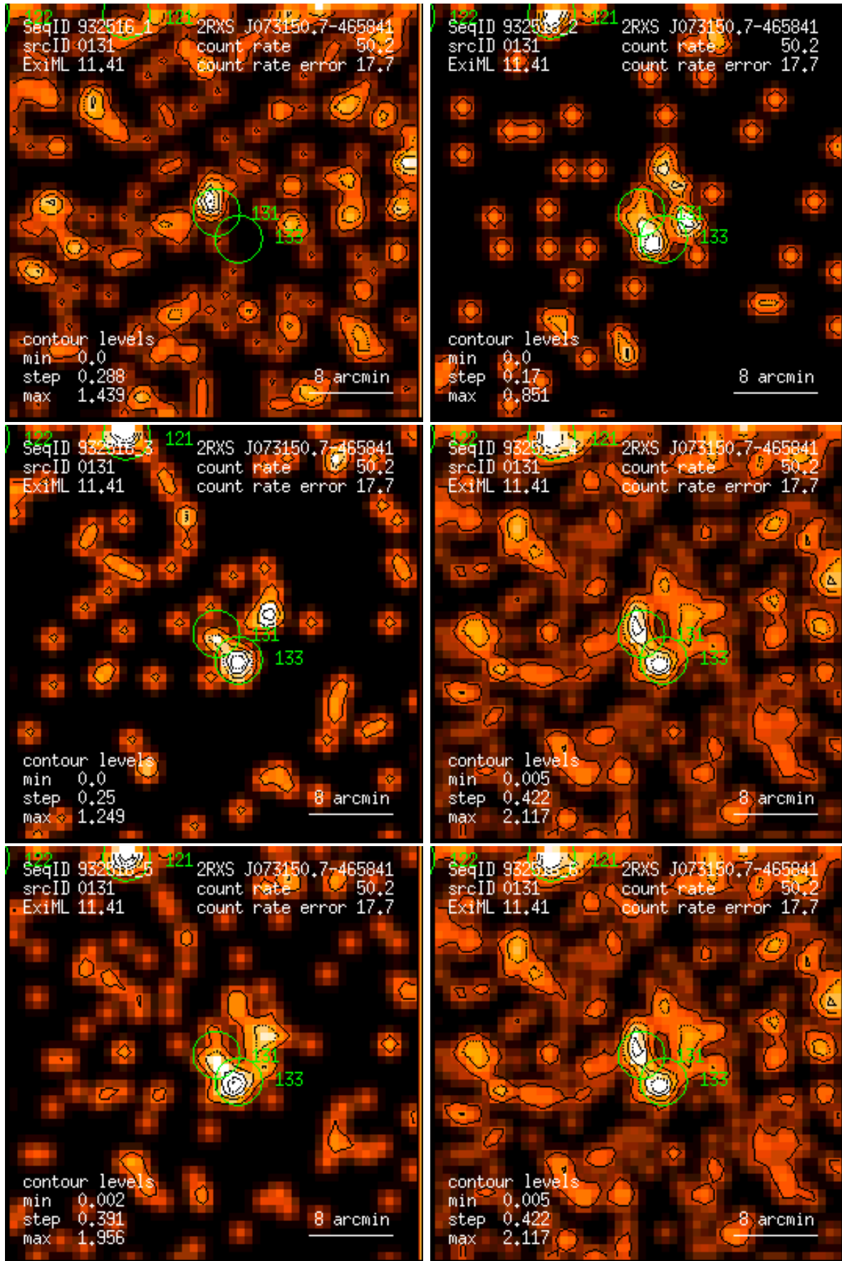
Figure 131: RASS 932516: detection 0131: band rate images, Gaussian filter: (1) PSPC channels 11 – 41, (2) 52 – 90, (3) 91 – 201, (4) 11 – 235, (5) 52 – 201, (6) 11 – 201. Broad band rates in counts/ks. Band rate contour levels in counts/ks/arcmin 2 .
