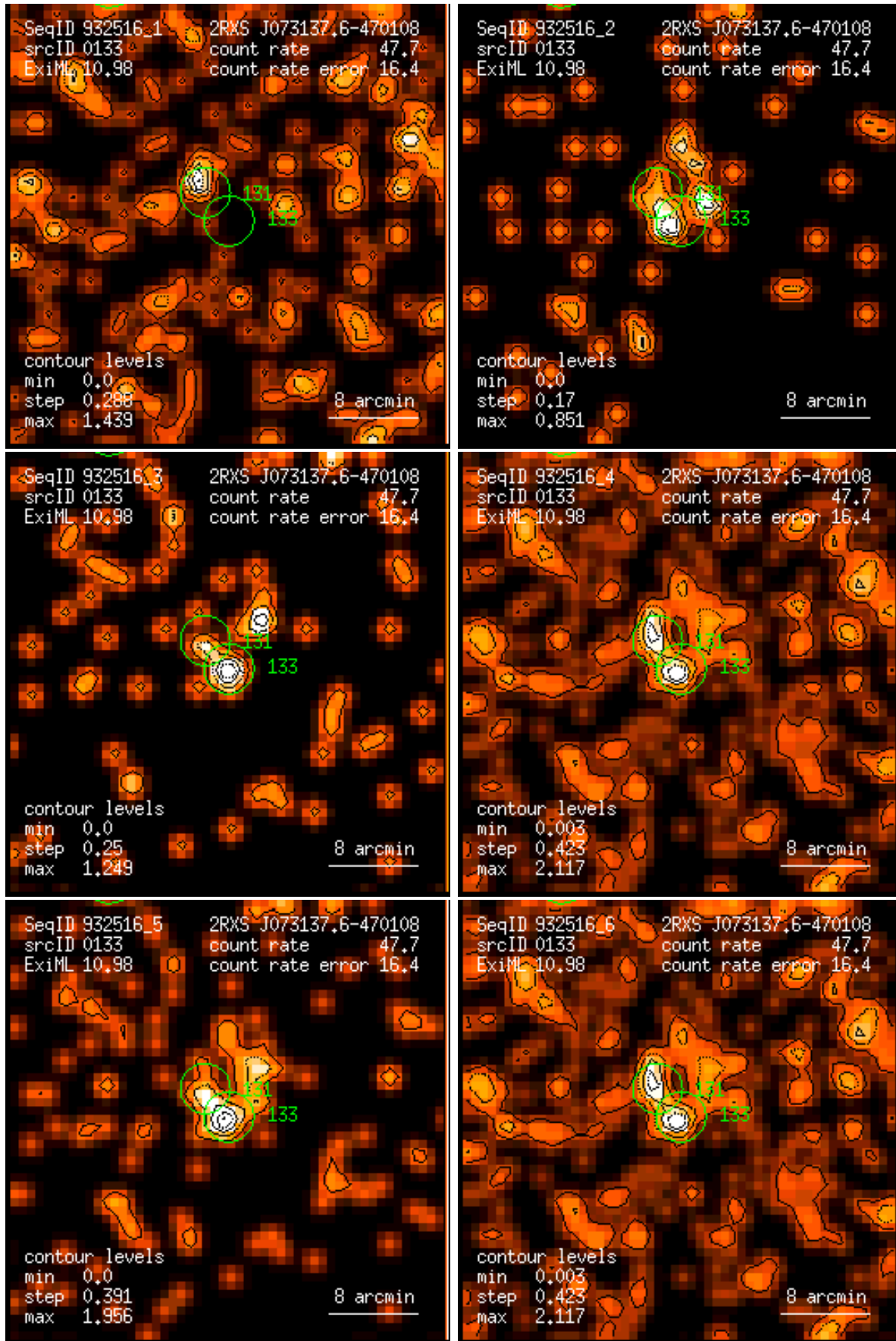
Figure 133: RASS 932516: detection 0133: band rate images, Gaussian filter: (1) PSPC channels 11 – 41, (2) 52 – 90, (3) 91 – 201, (4) 11 – 235, (5) 52 – 201, (6) 11 – 201. Broad band rates in counts/ks. Band rate contour levels in counts/ks/arcmin 2 .
