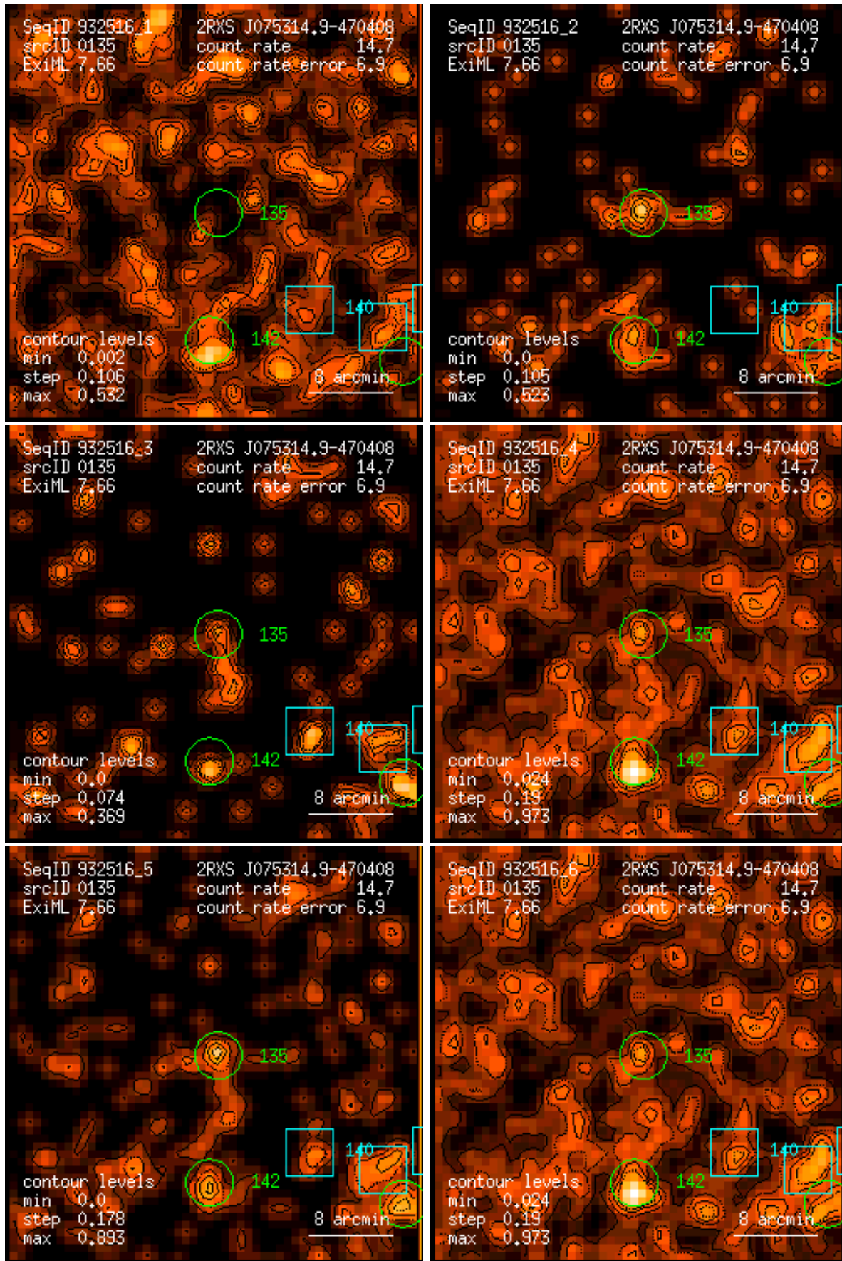
Figure 135: RASS 932516: detection 0135: band rate images, Gaussian filter: (1) PSPC channels 11 – 41, (2) 52 – 90, (3) 91 – 201, (4) 11 – 235, (5) 52 – 201, (6) 11 – 201. Broad band rates in counts/ks. Band rate contour levels in counts/ks/arcmin 2 .
