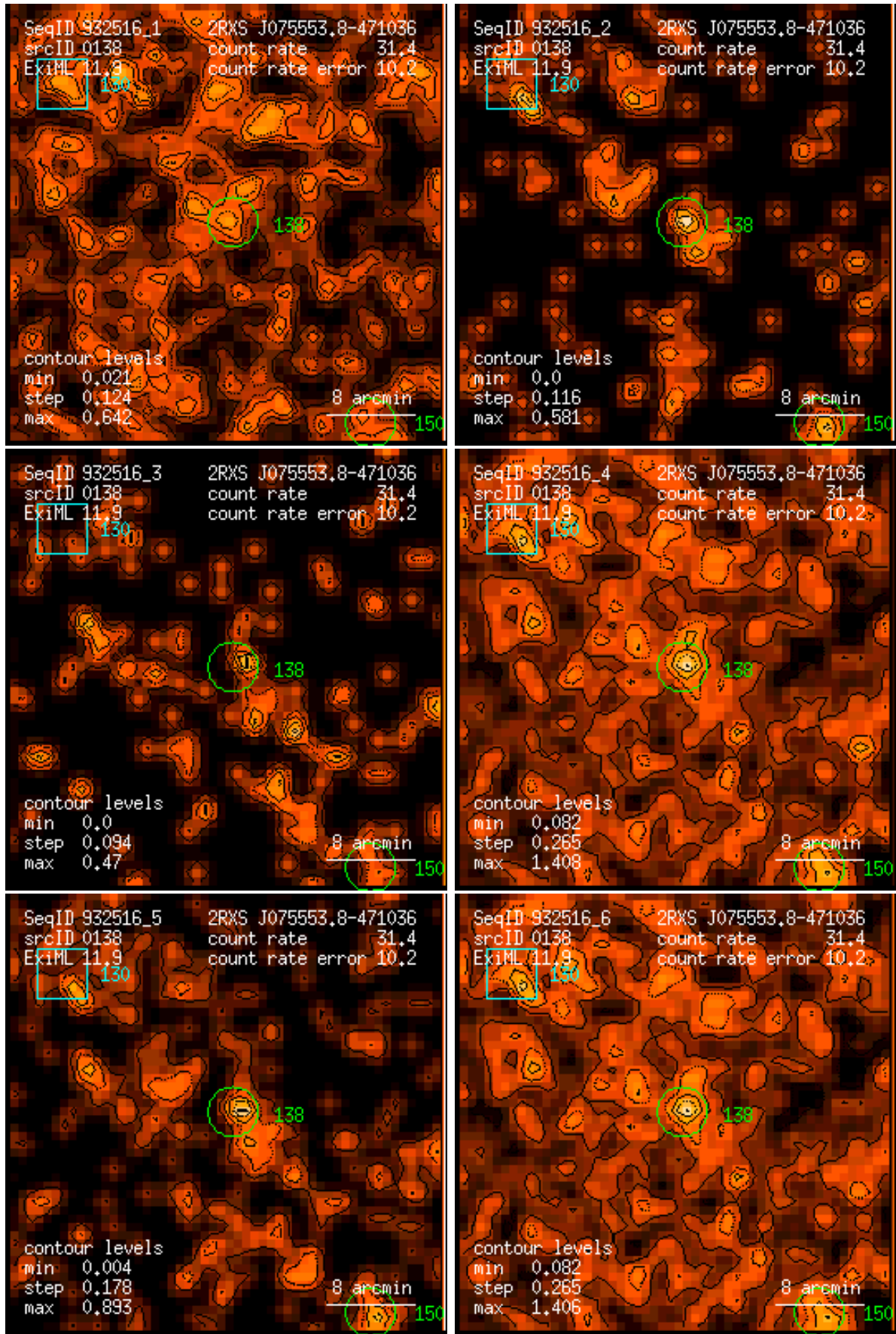
Figure 138: RASS 932516: detection 0138: band rate images, Gaussian filter: (1) PSPC channels 11 – 41, (2) 52 – 90, (3) 91 – 201, (4) 11 – 235, (5) 52 – 201, (6) 11 – 201. Broad band rates in counts/ks. Band rate contour levels in counts/ks/arcmin 2 .
