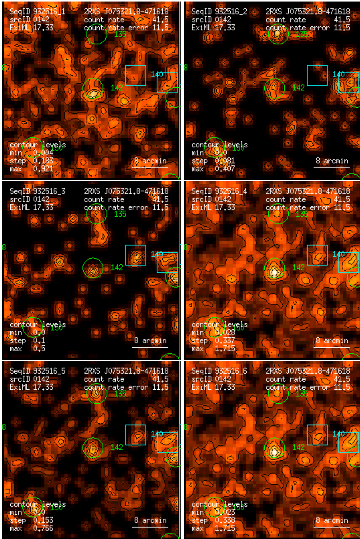
Figure 142: RASS 932516: detection 0142: band rate images, Gaussian filter: (1) PSPC channels 11 – 41, (2) 52 – 90, (3) 91 – 201, (4) 11 – 235, (5) 52 – 201, (6) 11 – 201. Broad band rates in counts/ks. Band rate contour levels in counts/ks/arcmin 2 .
