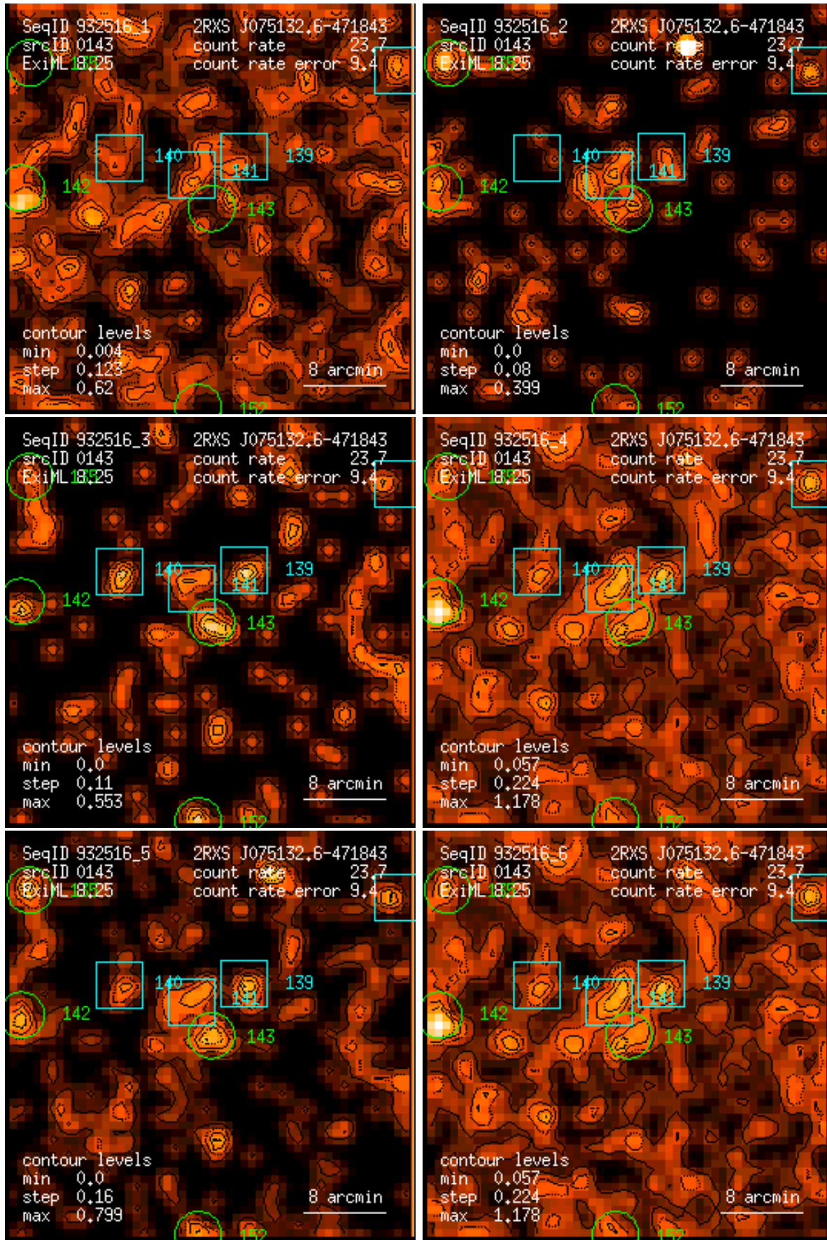
Figure 143: RASS 932516: detection 0143: band rate images, Gaussian filter: (1) PSPC channels 11 – 41, (2) 52 – 90, (3) 91 – 201, (4) 11 – 235, (5) 52 – 201, (6) 11 – 201. Broad band rates in counts/ks. Band rate contour levels in counts/ks/arcmin 2 .
