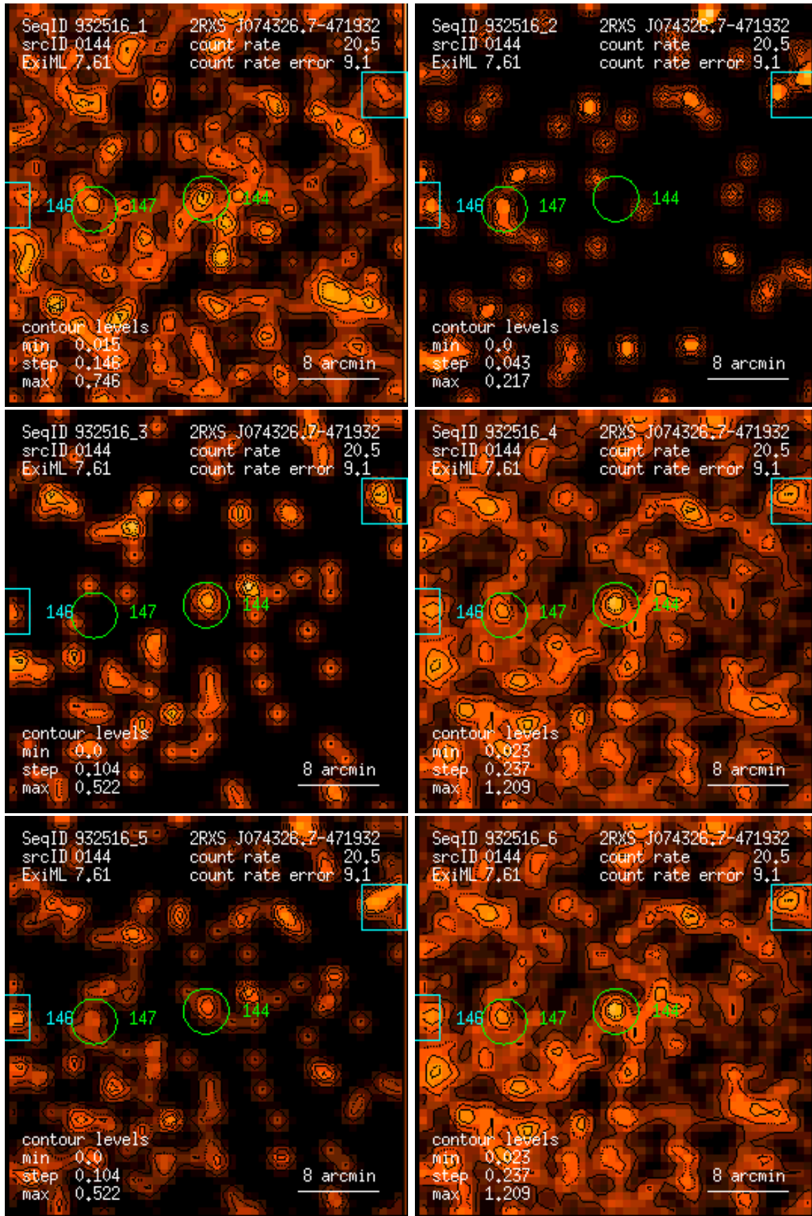
Figure 144: RASS 932516: detection 0144: band rate images, Gaussian filter: (1) PSPC channels 11 – 41, (2) 52 – 90, (3) 91 – 201, (4) 11 – 235, (5) 52 – 201, (6) 11 – 201. Broad band rates in counts/ks. Band rate contour levels in counts/ks/arcmin 2 .
