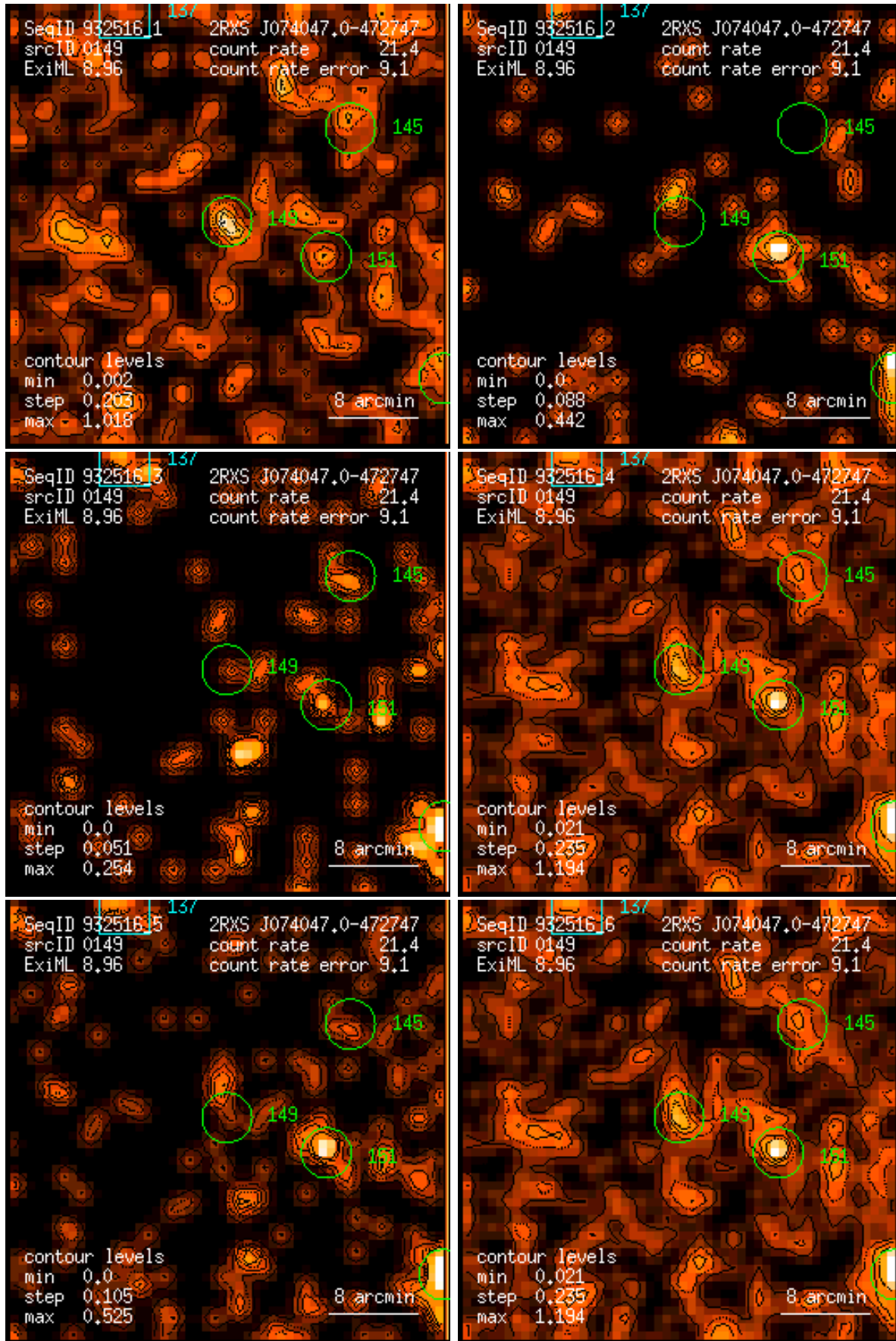
Figure 149: RASS 932516: detection 0149: band rate images, Gaussian filter: (1) PSPC channels 11 – 41, (2) 52 – 90, (3) 91 – 201, (4) 11 – 235, (5) 52 – 201, (6) 11 – 201. Broad band rates in counts/ks. Band rate contour levels in counts/ks/arcmin 2 .
