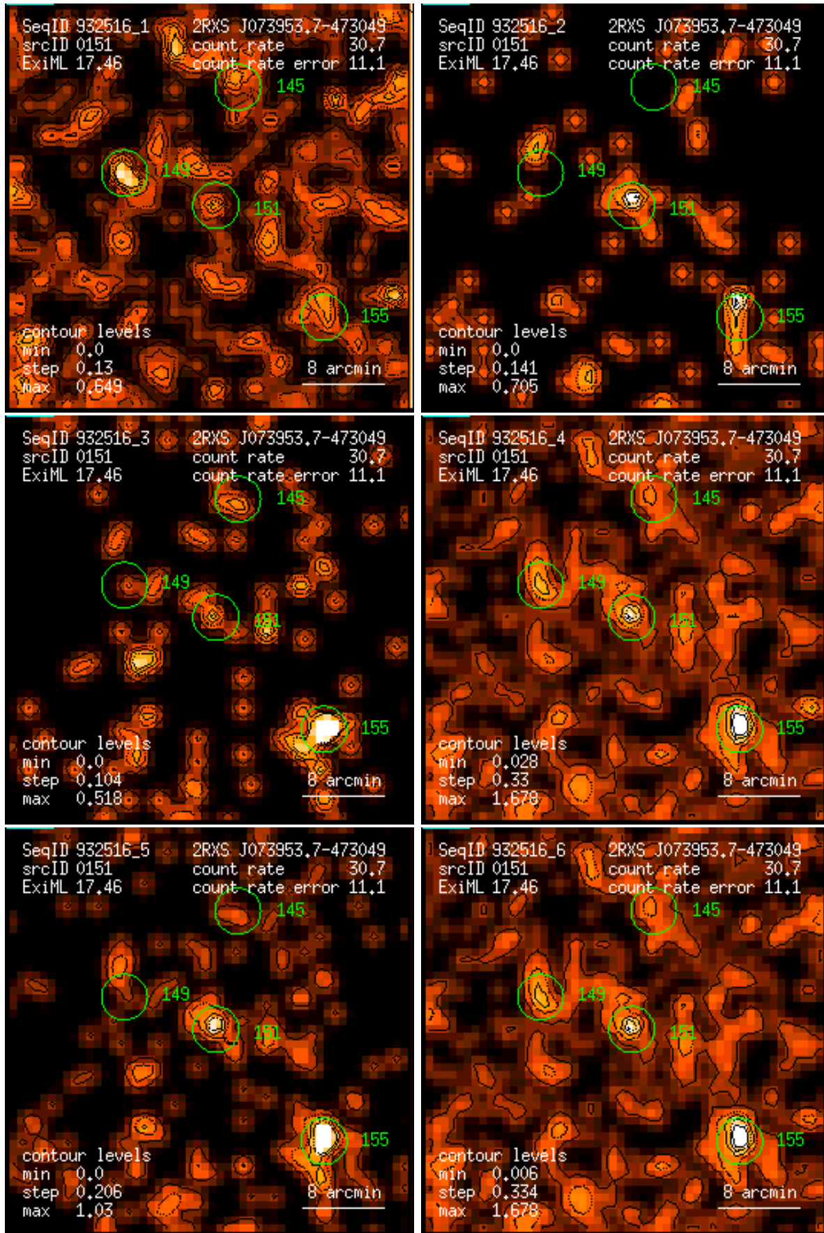
Figure 151: RASS 932516: detection 0151: band rate images, Gaussian filter: (1) PSPC channels 11 – 41, (2) 52 – 90, (3) 91 – 201, (4) 11 – 235, (5) 52 – 201, (6) 11 – 201. Broad band rates in counts/ks. Band rate contour levels in counts/ks/arcmin 2 .
