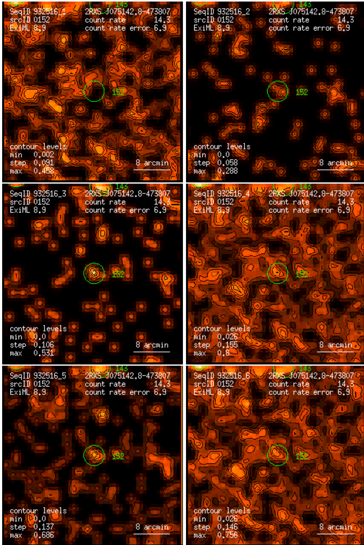
Figure 152: RASS 932516: detection 0152: band rate images, Gaussian filter: (1) PSPC channels 11 – 41, (2) 52 – 90, (3) 91 – 201, (4) 11 – 235, (5) 52 – 201, (6) 11 – 201. Broad band rates in counts/ks. Band rate contour levels in counts/ks/arcmin 2 .
