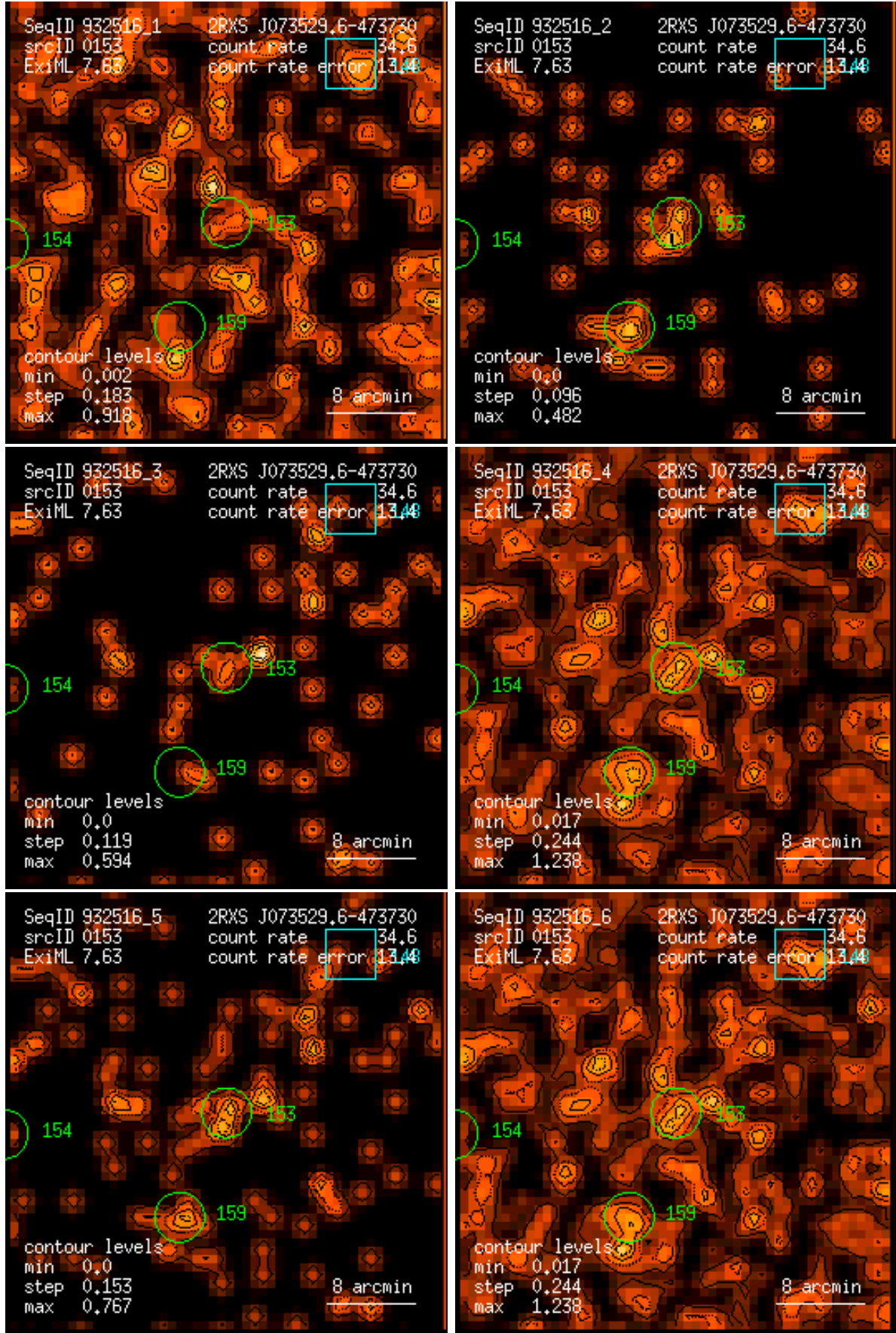
Figure 153: RASS 932516: detection 0153: band rate images, Gaussian filter: (1) PSPC channels 11 – 41, (2) 52 – 90, (3) 91 – 201, (4) 11 – 235, (5) 52 – 201, (6) 11 – 201. Broad band rates in counts/ks. Band rate contour levels in counts/ks/arcmin 2 .
