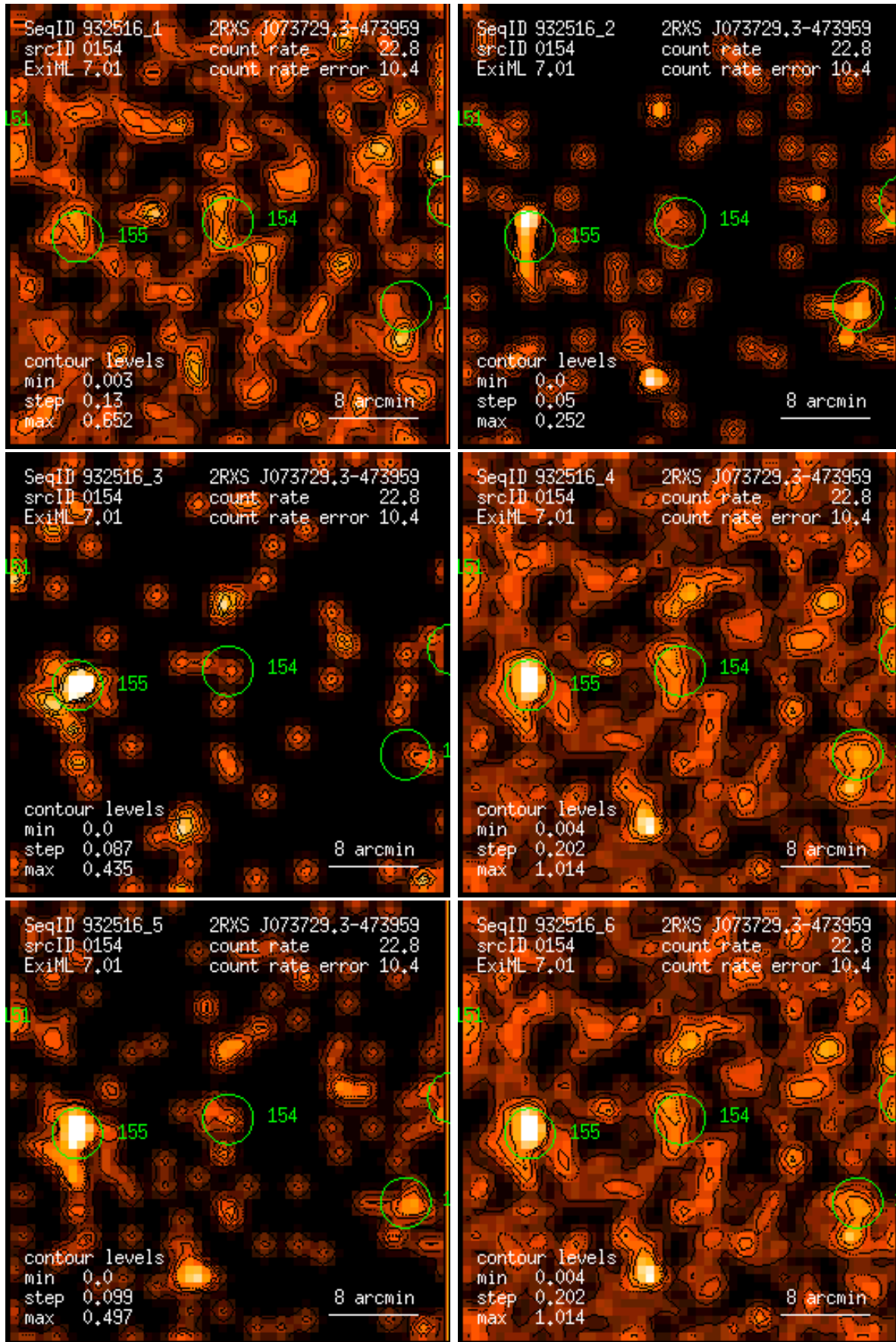
Figure 154: RASS 932516: detection 0154: band rate images, Gaussian filter: (1) PSPC channels 11 – 41, (2) 52 – 90, (3) 91 – 201, (4) 11 – 235, (5) 52 – 201, (6) 11 – 201. Broad band rates in counts/ks. Band rate contour levels in counts/ks/arcmin 2 .
