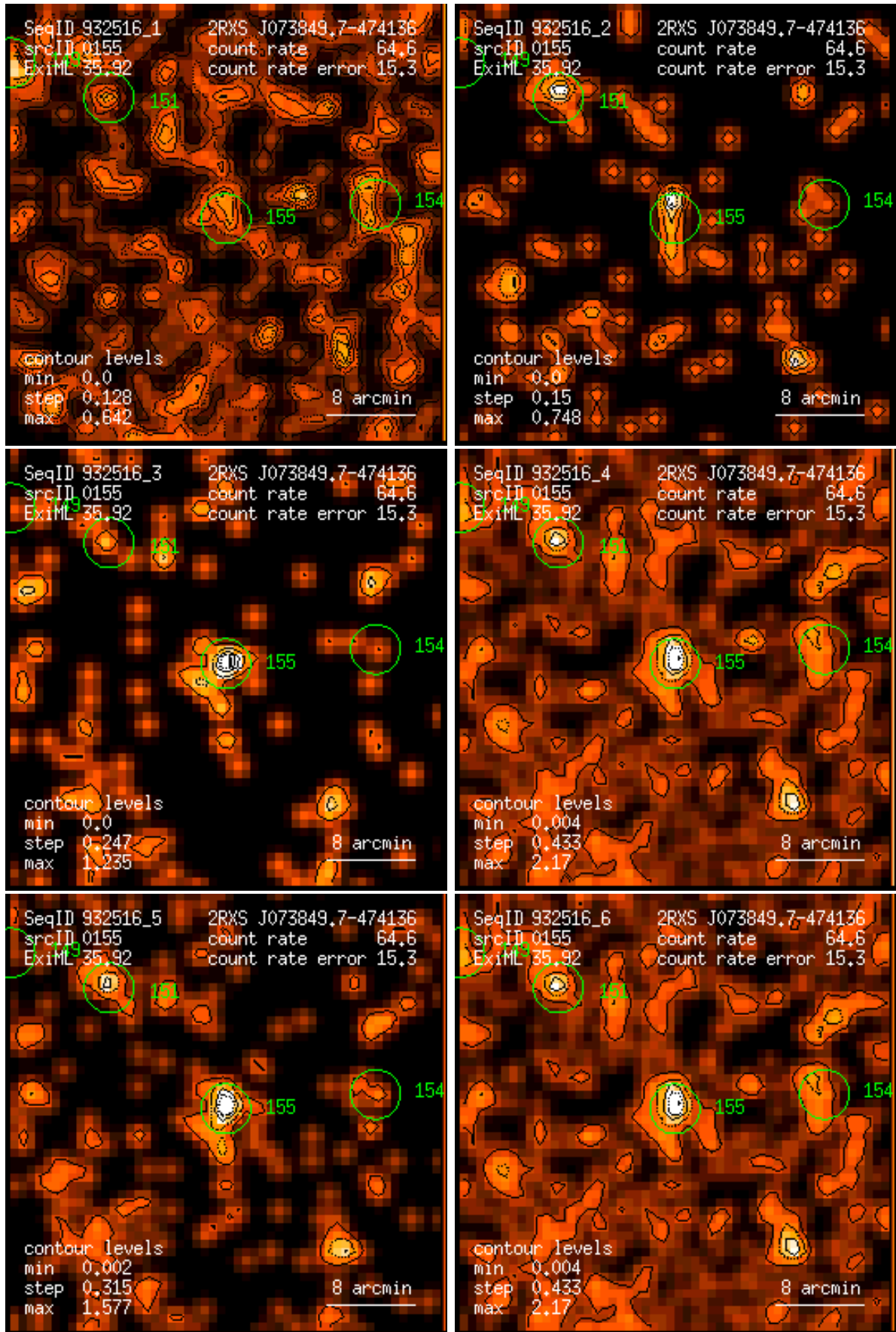
Figure 155: RASS 932516: detection 0155: band rate images, Gaussian filter: (1) PSPC channels 11 – 41, (2) 52 – 90, (3) 91 – 201, (4) 11 – 235, (5) 52 – 201, (6) 11 – 201. Broad band rates in counts/ks. Band rate contour levels in counts/ks/arcmin 2 .
