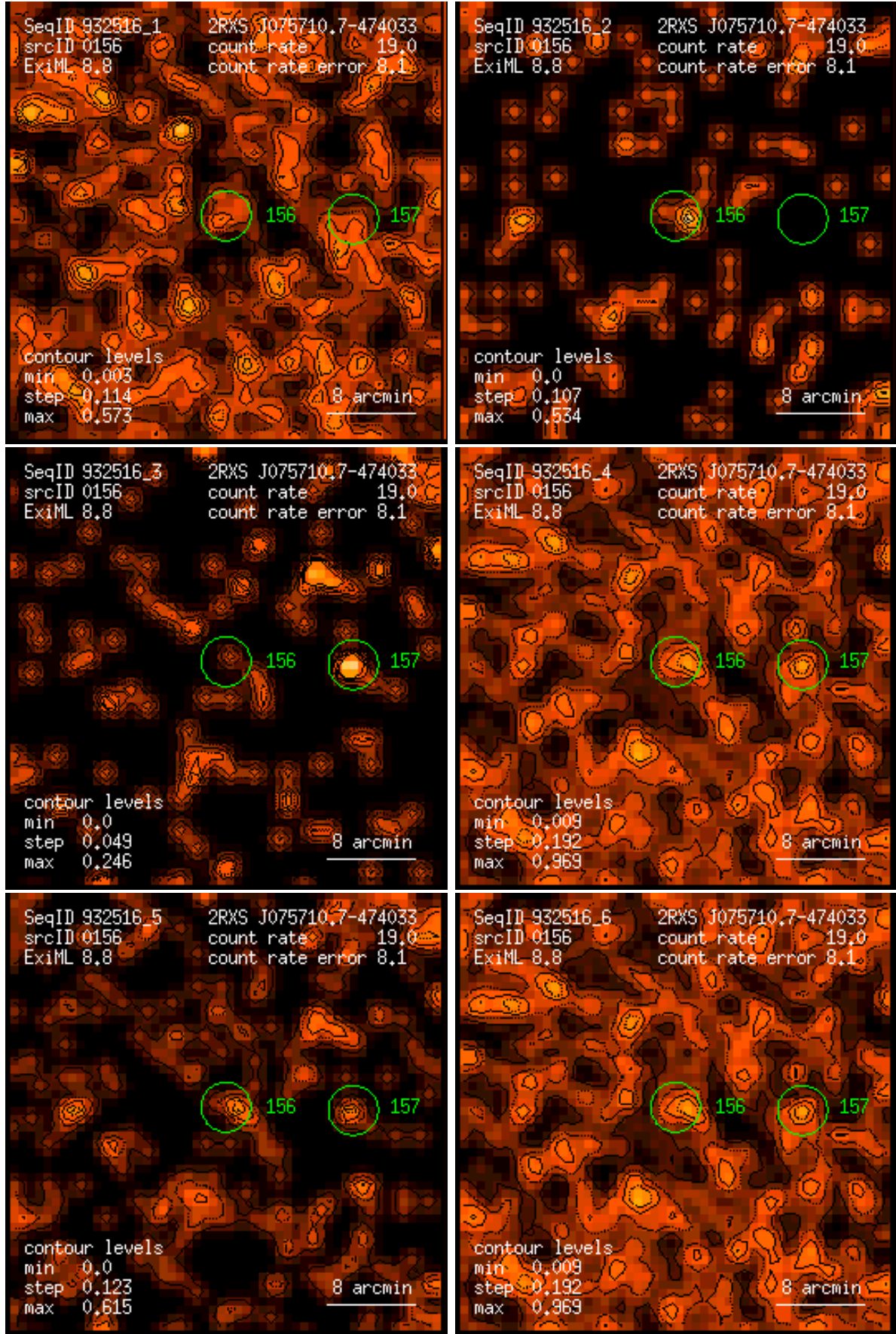
Figure 156: RASS 932516: detection 0156: band rate images, Gaussian filter: (1) PSPC channels 11 – 41, (2) 52 – 90, (3) 91 – 201, (4) 11 – 235, (5) 52 – 201, (6) 11 – 201. Broad band rates in counts/ks. Band rate contour levels in counts/ks/arcmin 2 .
