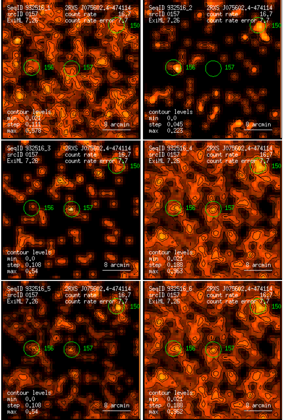
Figure 157: RASS 932516: detection 0157: band rate images, Gaussian filter: (1) PSPC channels 11 – 41, (2) 52 – 90, (3) 91 – 201, (4) 11 – 235, (5) 52 – 201, (6) 11 – 201. Broad band rates in counts/ks. Band rate contour levels in counts/ks/arcmin 2 .
