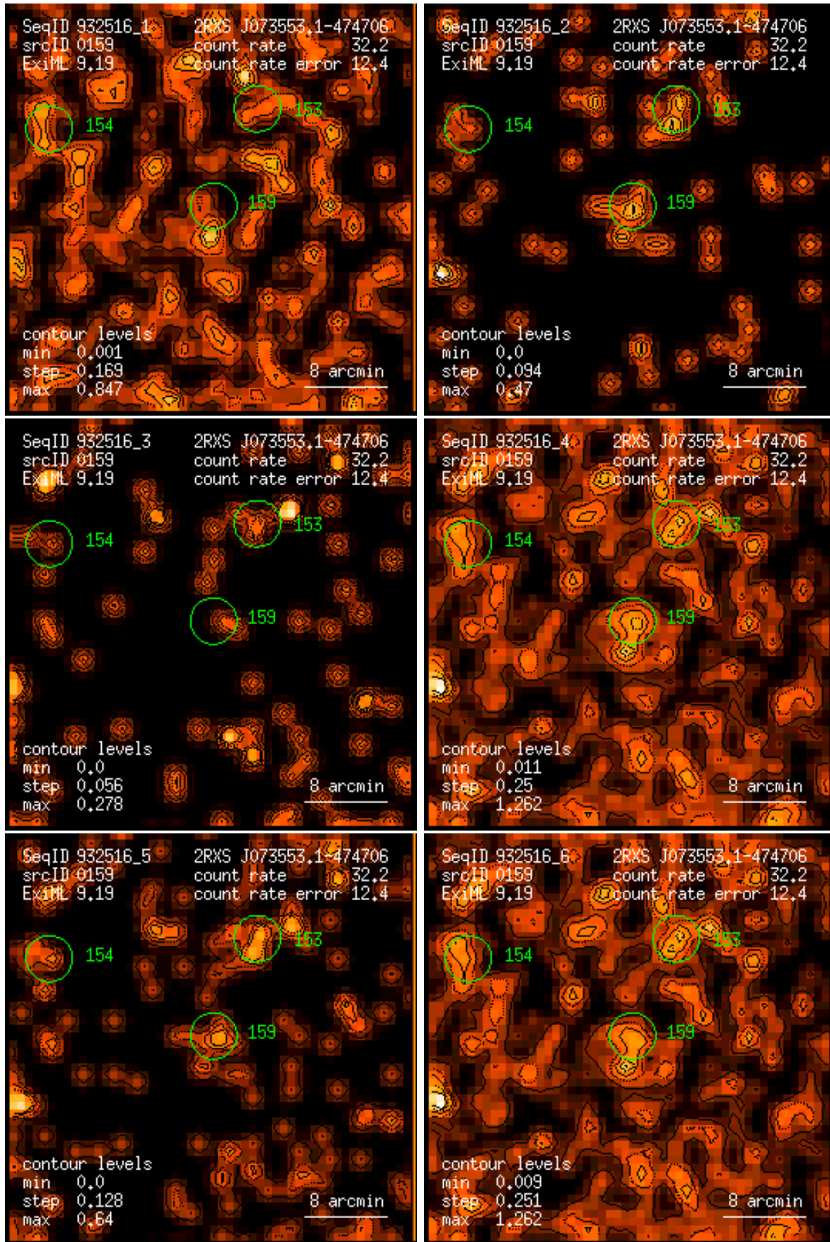
Figure 159: RASS 932516: detection 0159: band rate images, Gaussian filter: (1) PSPC channels 11 – 41, (2) 52 – 90, (3) 91 – 201, (4) 11 – 235, (5) 52 – 201, (6) 11 – 201. Broad band rates in counts/ks. Band rate contour levels in counts/ks/arcmin 2 .
