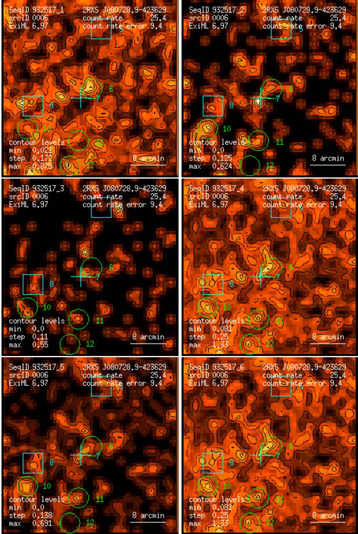
Figure 6: RASS 932517: detection 0006: band rate images, Gaussian filter: (1) PSPC channels 11 – 41, (2) 52 – 90, (3) 91 – 201, (4) 11 – 235, (5) 52 – 201, (6) 11 – 201. Broad band rates in counts/ks. Band rate contour levels in counts/ks/arcmin 2 .
