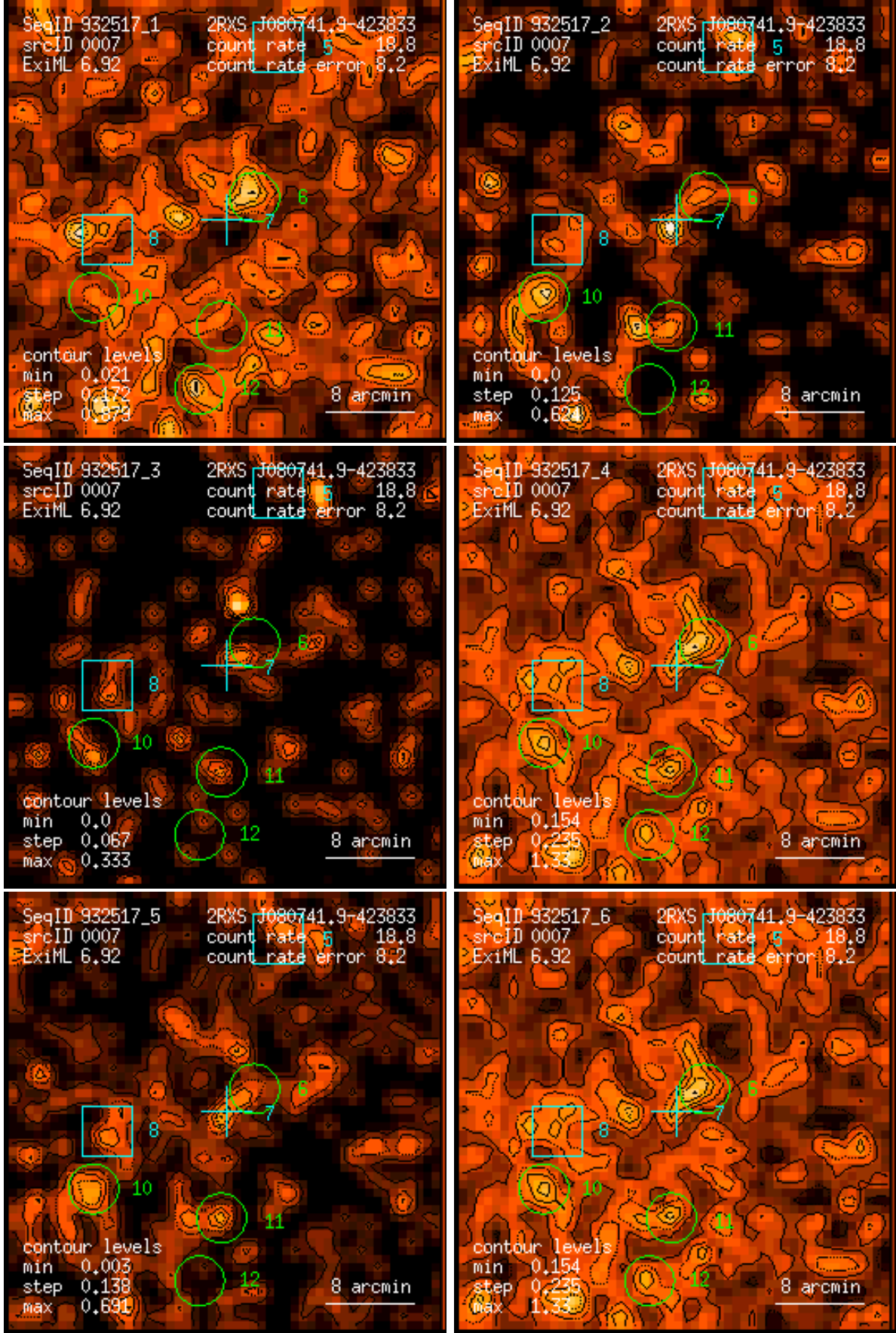
Figure 7: RASS 932517: detection 0007: band rate images, Gaussian filter: (1) PSPC channels 11 – 41, (2) 52 – 90, (3) 91 – 201, (4) 11 – 235, (5) 52 – 201, (6) 11 – 201. Broad band rates in counts/ks. Band rate contour levels in counts/ks/arcmin 2 .
