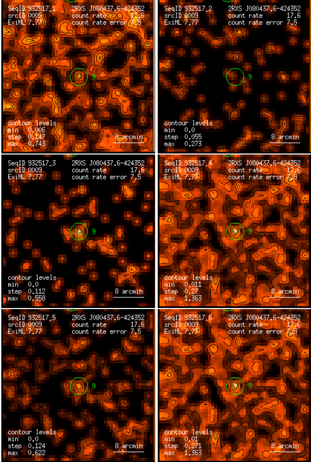
Figure 9: RASS 932517: detection 0009: band rate images, Gaussian filter: (1) PSPC channels 11 – 41, (2) 52 – 90, (3) 91 – 201, (4) 11 – 235, (5) 52 – 201, (6) 11 – 201. Broad band rates in counts/ks. Band rate contour levels in counts/ks/arcmin 2 .
