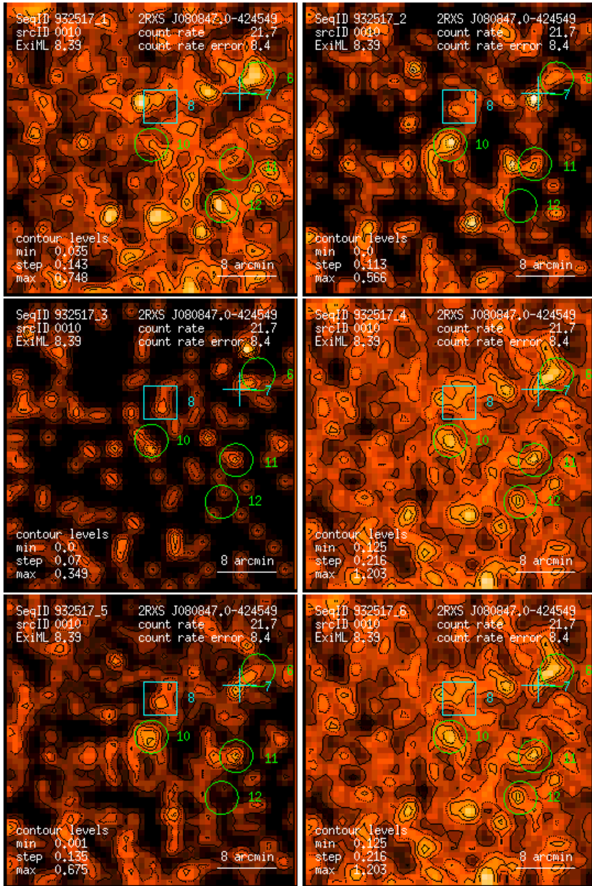
Figure 10: RASS 932517: detection 0010: band rate images, Gaussian filter: (1) PSPC channels 11 – 41, (2) 52 – 90, (3) 91 – 201, (4) 11 – 235, (5) 52 – 201, (6) 11 – 201. Broad band rates in counts/ks. Band rate contour levels in counts/ks/arcmin 2 .
