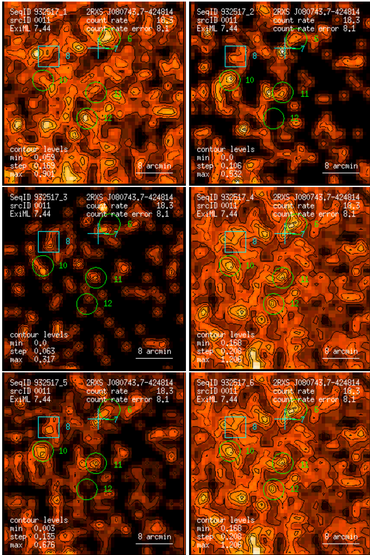
Figure 11: RASS 932517: detection 0011: band rate images, Gaussian filter: (1) PSPC channels 11 – 41, (2) 52 – 90, (3) 91 – 201, (4) 11 – 235, (5) 52 – 201, (6) 11 – 201. Broad band rates in counts/ks. Band rate contour levels in counts/ks/arcmin 2 .
