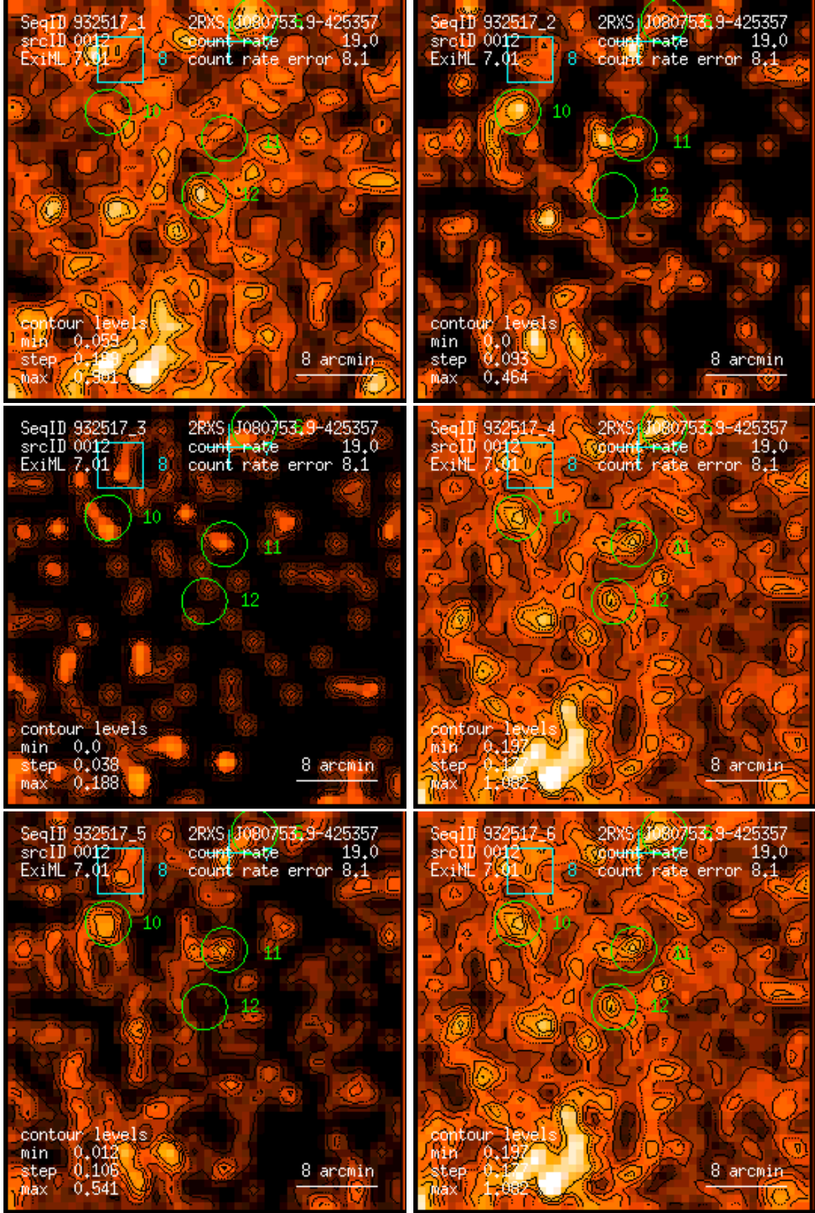
Figure 12: RASS 932517: detection 0012: band rate images, Gaussian filter: (1) PSPC channels 11 – 41, (2) 52 – 90, (3) 91 – 201, (4) 11 – 235, (5) 52 – 201, (6) 11 – 201. Broad band rates in counts/ks. Band rate contour levels in counts/ks/arcmin 2 .
