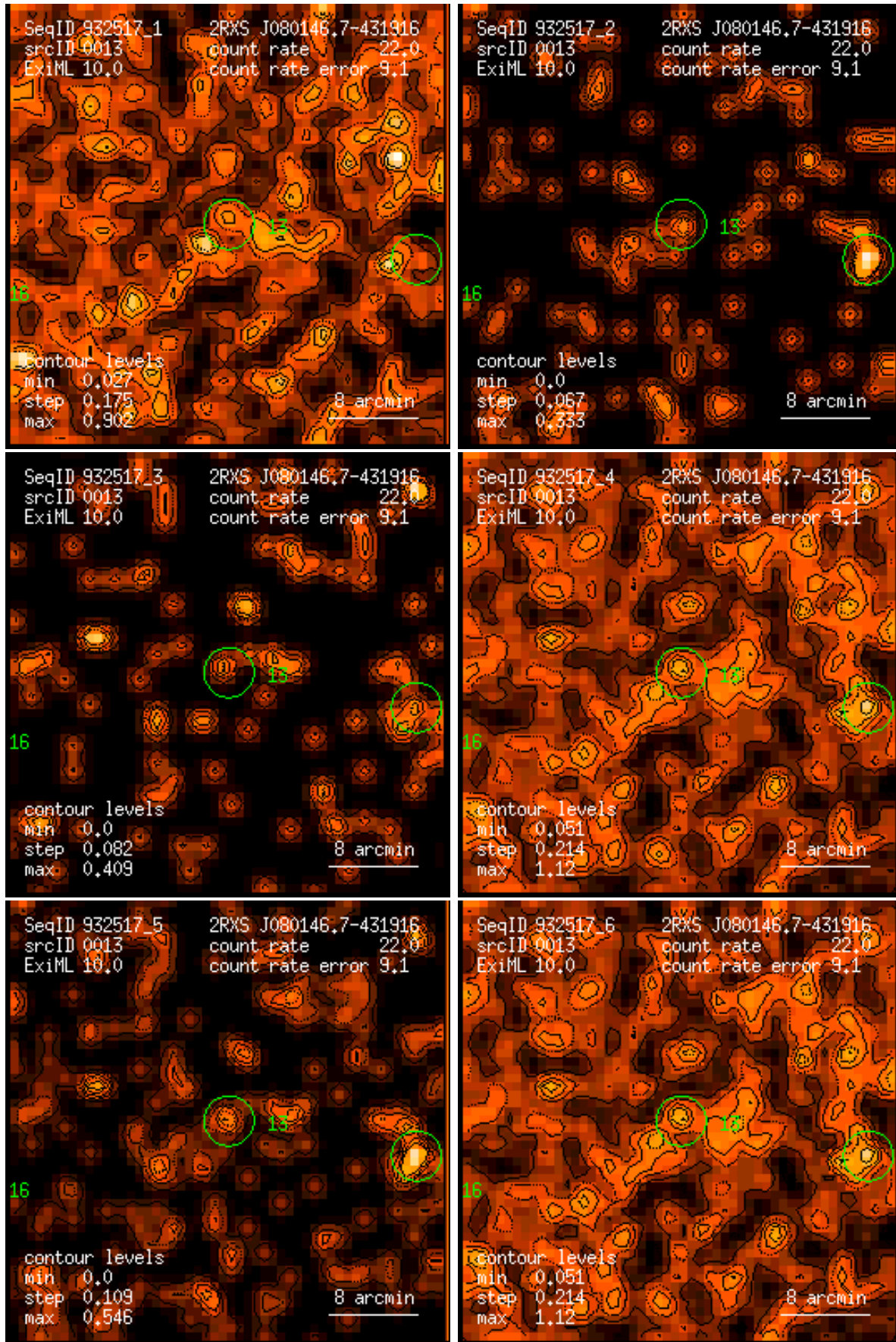
Figure 13: RASS 932517: detection 0013: band rate images, Gaussian filter: (1) PSPC channels 11 – 41, (2) 52 – 90, (3) 91 – 201, (4) 11 – 235, (5) 52 – 201, (6) 11 – 201. Broad band rates in counts/ks. Band rate contour levels in counts/ks/arcmin 2 .
