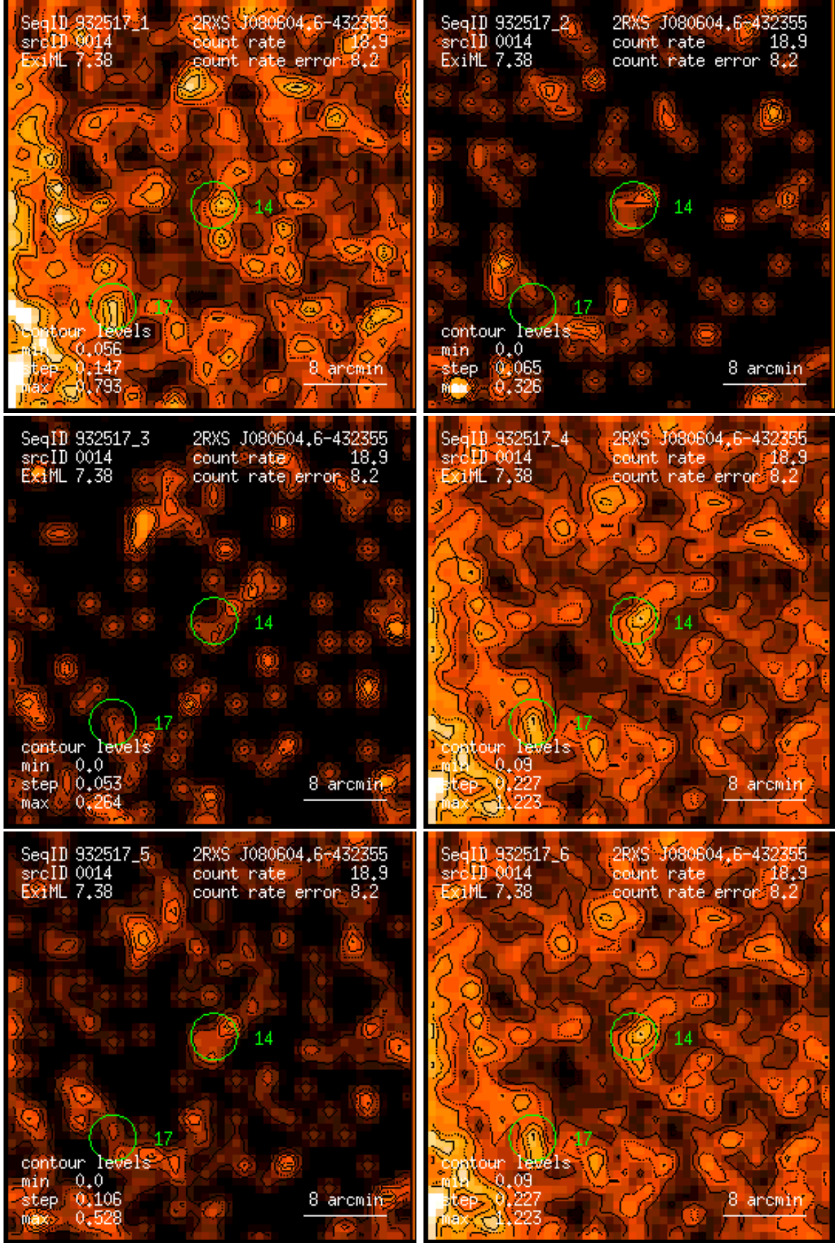
Figure 14: RASS 932517: detection 0014: band rate images, Gaussian filter: (1) PSPC channels 11 – 41, (2) 52 – 90, (3) 91 – 201, (4) 11 – 235, (5) 52 – 201, (6) 11 – 201. Broad band rates in counts/ks. Band rate contour levels in counts/ks/arcmin 2 .
