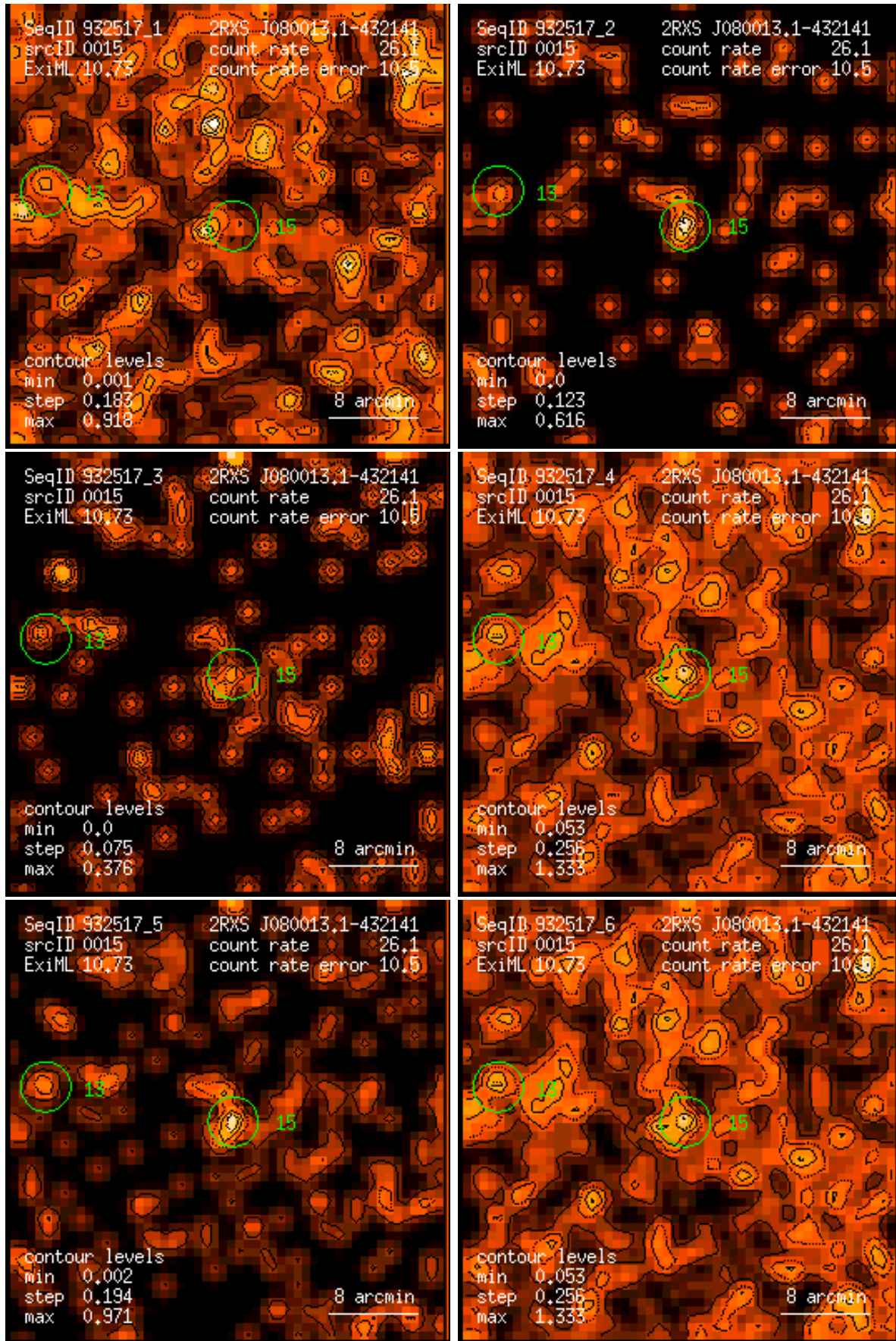
Figure 15: RASS 932517: detection 0015: band rate images, Gaussian filter: (1) PSPC channels 11 – 41, (2) 52 – 90, (3) 91 – 201, (4) 11 – 235, (5) 52 – 201, (6) 11 – 201. Broad band rates in counts/ks. Band rate contour levels in counts/ks/arcmin 2 .
