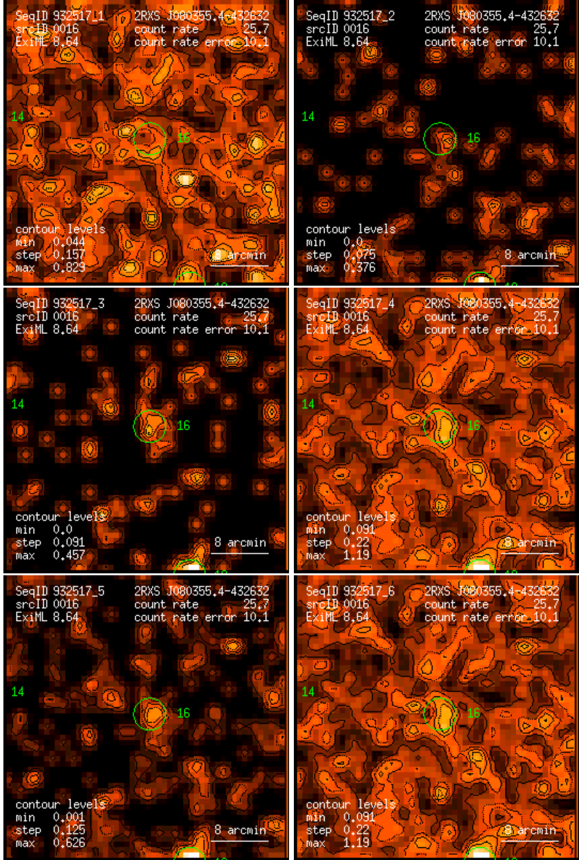
Figure 16: RASS 932517: detection 0016: band rate images, Gaussian filter: (1) PSPC channels 11 – 41, (2) 52 – 90, (3) 91 – 201, (4) 11 – 235, (5) 52 – 201, (6) 11 – 201. Broad band rates in counts/ks. Band rate contour levels in counts/ks/arcmin 2 .
