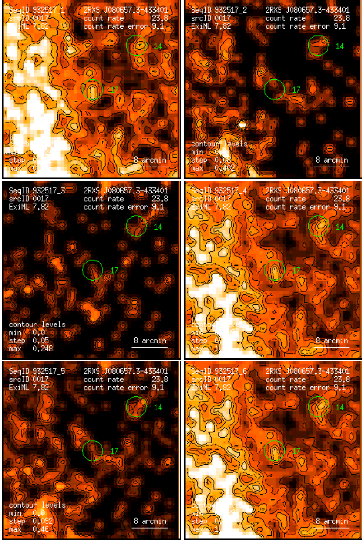
Figure 17: RASS 932517: detection 0017: band rate images, Gaussian filter: (1) PSPC channels 11 – 41, (2) 52 – 90, (3) 91 – 201, (4) 11 – 235, (5) 52 – 201, (6) 11 – 201. Broad band rates in counts/ks. Band rate contour levels in counts/ks/arcmin 2 .
