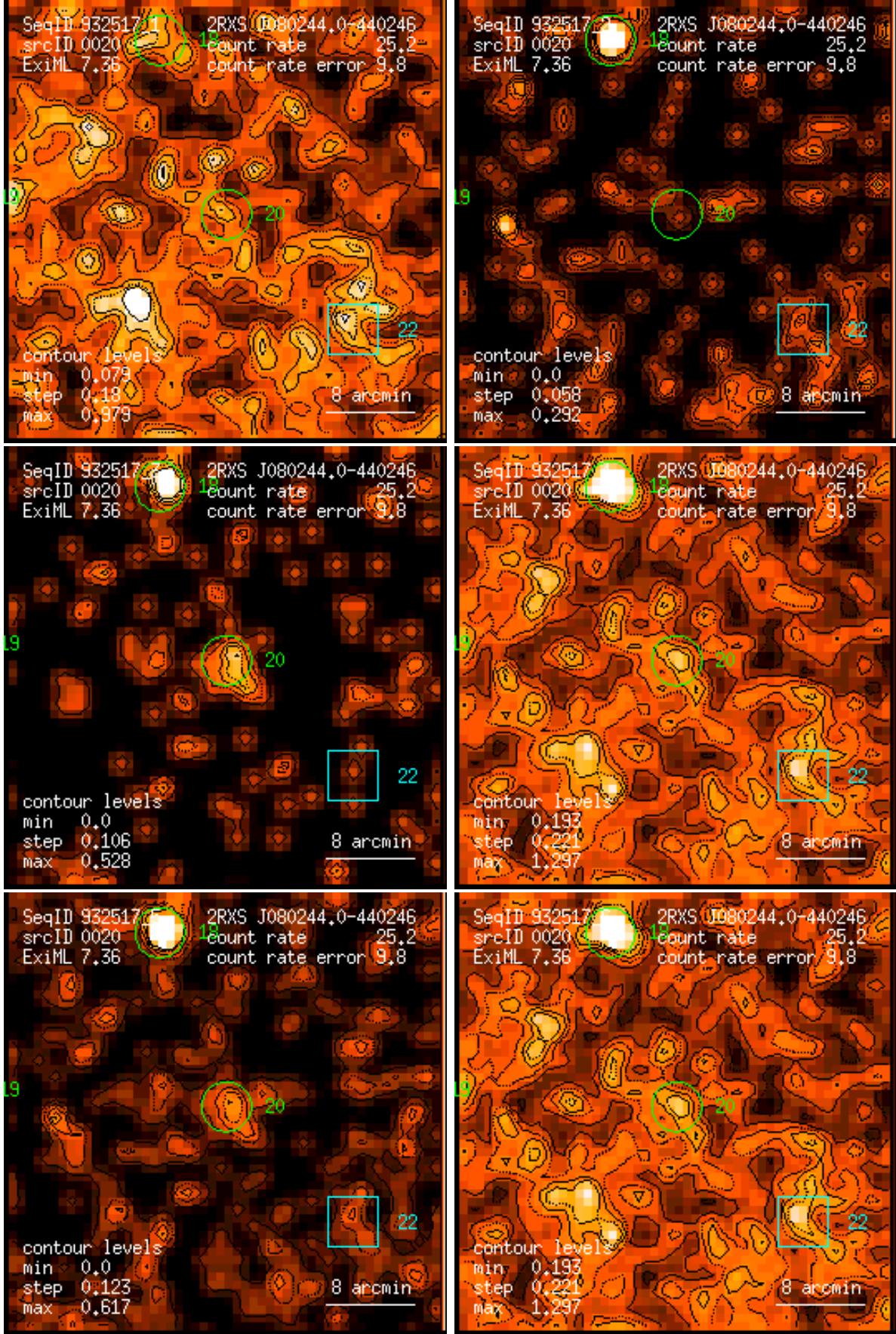
Figure 20: RASS 932517: detection 0020: band rate images, Gaussian filter: (1) PSPC channels 11 – 41, (2) 52 – 90, (3) 91 – 201, (4) 11 – 235, (5) 52 – 201, (6) 11 – 201. Broad band rates in counts/ks. Band rate contour levels in counts/ks/arcmin 2 .
