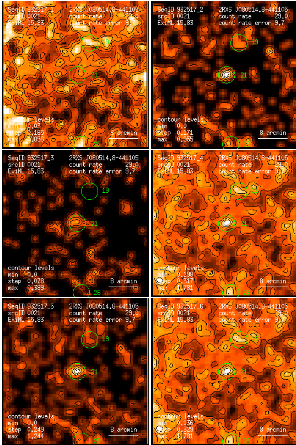
Figure 21: RASS 932517: detection 0021: band rate images, Gaussian filter: (1) PSPC channels 11 – 41, (2) 52 – 90, (3) 91 – 201, (4) 11 – 235, (5) 52 – 201, (6) 11 – 201. Broad band rates in counts/ks. Band rate contour levels in counts/ks/arcmin 2 .
