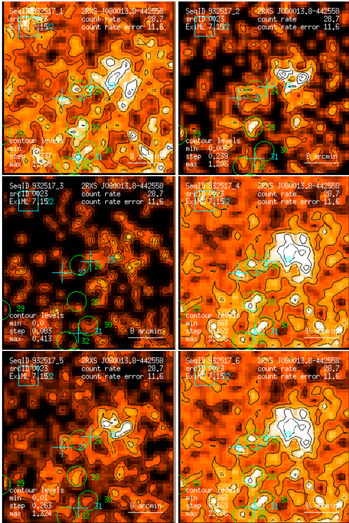
Figure 23: RASS 932517: detection 0023: band rate images, Gaussian filter: (1) PSPC channels 11 – 41, (2) 52 – 90, (3) 91 – 201, (4) 11 – 235, (5) 52 – 201, (6) 11 – 201. Broad band rates in counts/ks. Band rate contour levels in counts/ks/arcmin 2 .
