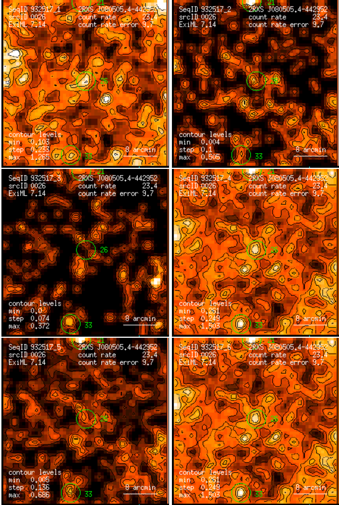
Figure 26: RASS 932517: detection 0026: band rate images, Gaussian filter: (1) PSPC channels 11 – 41, (2) 52 – 90, (3) 91 – 201, (4) 11 – 235, (5) 52 – 201, (6) 11 – 201. Broad band rates in counts/ks. Band rate contour levels in counts/ks/arcmin 2 .
