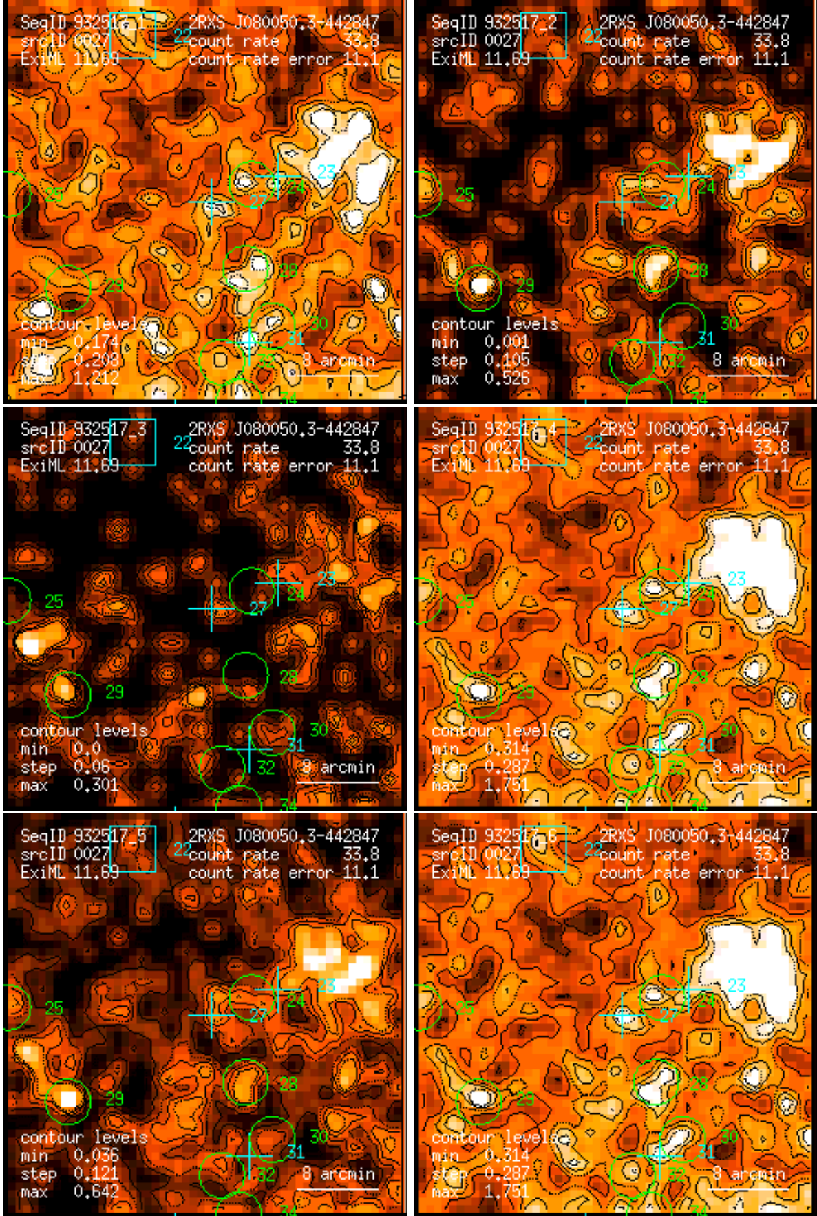
Figure 27: RASS 932517: detection 0027: band rate images, Gaussian filter: (1) PSPC channels 11 – 41, (2) 52 – 90, (3) 91 – 201, (4) 11 – 235, (5) 52 – 201, (6) 11 – 201. Broad band rates in counts/ks. Band rate contour levels in counts/ks/arcmin 2 .
