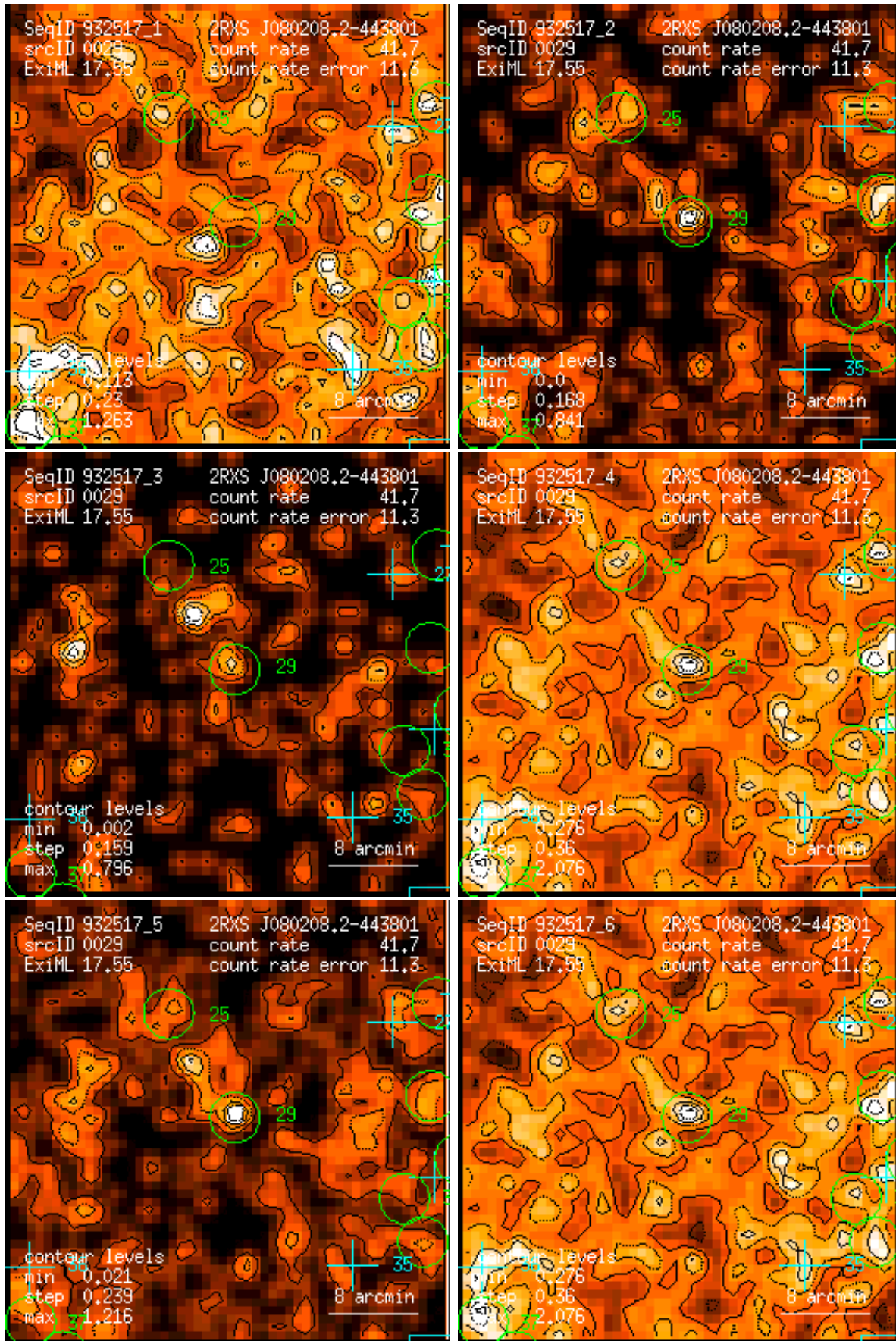
Figure 29: RASS 932517: detection 0029: band rate images, Gaussian filter: (1) PSPC channels 11 – 41, (2) 52 – 90, (3) 91 – 201, (4) 11 – 235, (5) 52 – 201, (6) 11 – 201. Broad band rates in counts/ks. Band rate contour levels in counts/ks/arcmin 2 .
