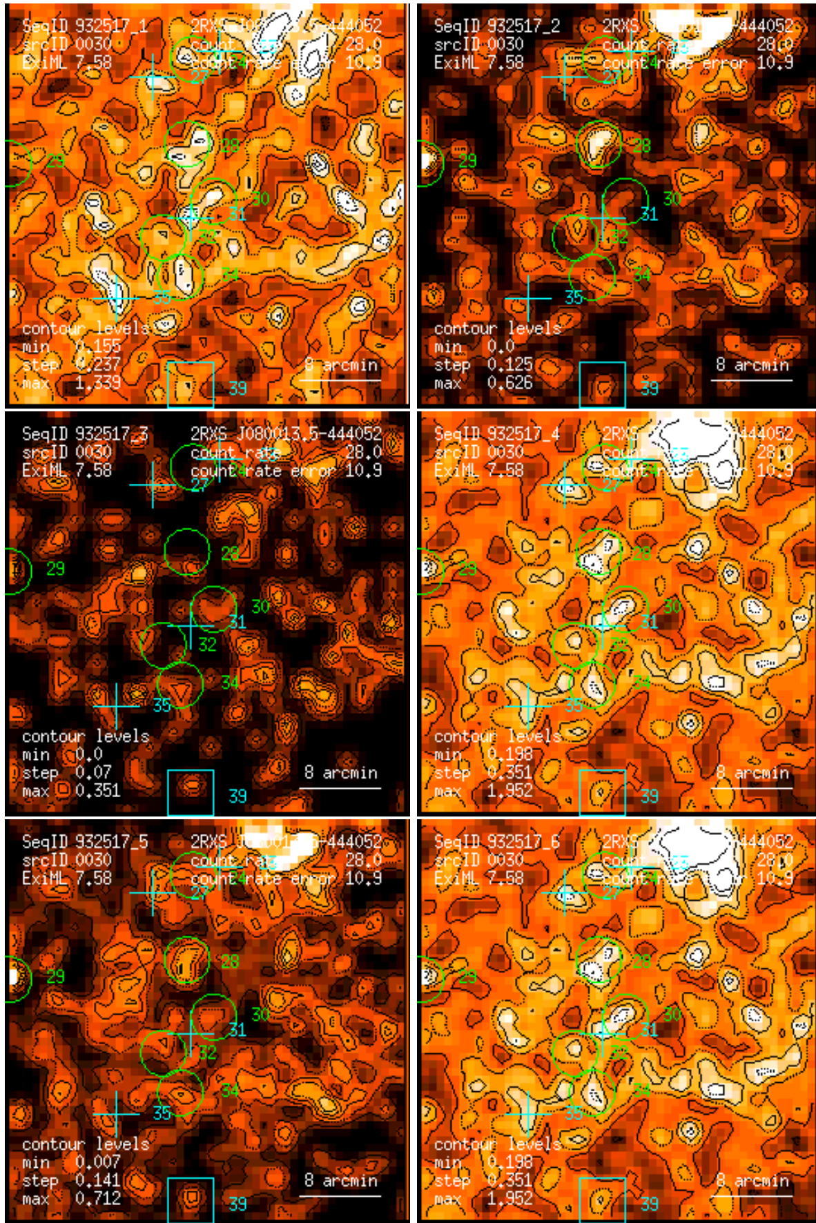
Figure 30: RASS 932517: detection 0030: band rate images, Gaussian filter: (1) PSPC channels 11 – 41, (2) 52 – 90, (3) 91 – 201, (4) 11 – 235, (5) 52 – 201, (6) 11 – 201. Broad band rates in counts/ks. Band rate contour levels in counts/ks/arcmin 2 .
