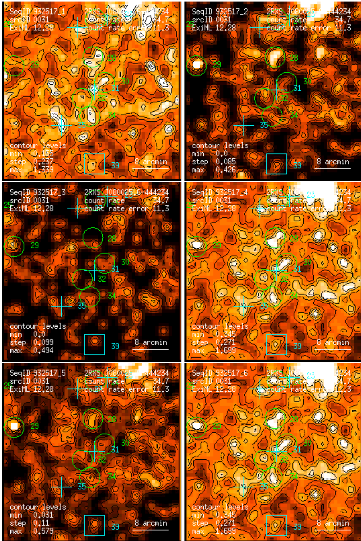
Figure 31: RASS 932517: detection 0031: band rate images, Gaussian filter: (1) PSPC channels 11 – 41, (2) 52 – 90, (3) 91 – 201, (4) 11 – 235, (5) 52 – 201, (6) 11 – 201. Broad band rates in counts/ks. Band rate contour levels in counts/ks/arcmin 2 .
