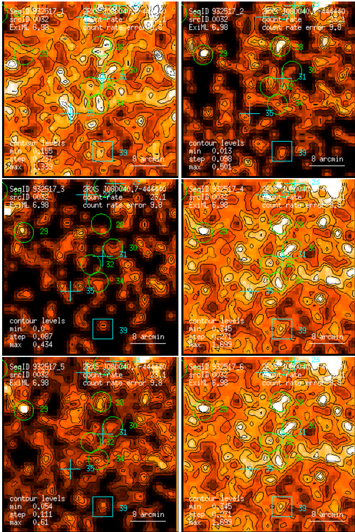
Figure 32: RASS 932517: detection 0032: band rate images, Gaussian filter: (1) PSPC channels 11 – 41, (2) 52 – 90, (3) 91 – 201, (4) 11 – 235, (5) 52 – 201, (6) 11 – 201. Broad band rates in counts/ks. Band rate contour levels in counts/ks/arcmin 2 .
