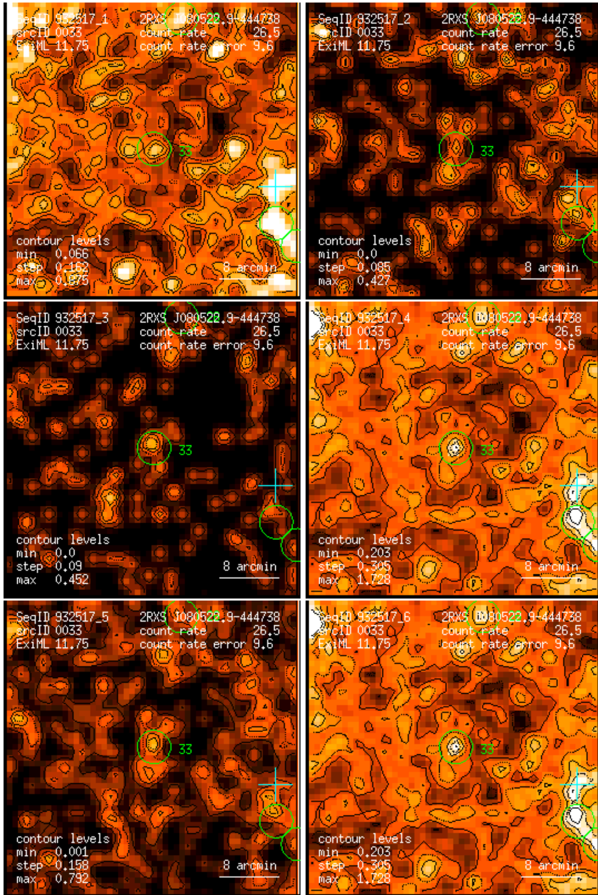
Figure 33: RASS 932517: detection 0033: band rate images, Gaussian filter: (1) PSPC channels 11 – 41, (2) 52 – 90, (3) 91 – 201, (4) 11 – 235, (5) 52 – 201, (6) 11 – 201. Broad band rates in counts/ks. Band rate contour levels in counts/ks/arcmin 2 .
