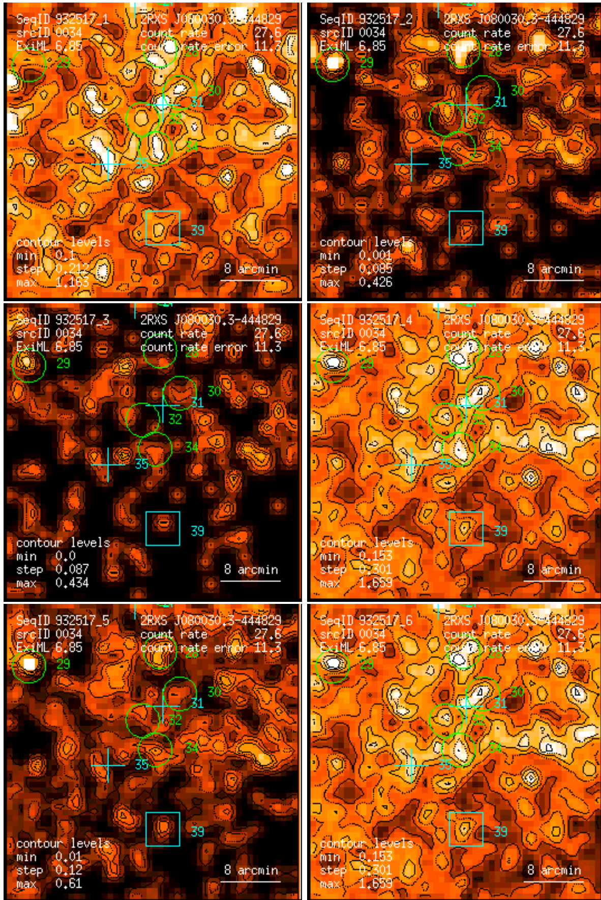
Figure 34: RASS 932517: detection 0034: band rate images, Gaussian filter: (1) PSPC channels 11 – 41, (2) 52 – 90, (3) 91 – 201, (4) 11 – 235, (5) 52 – 201, (6) 11 – 201. Broad band rates in counts/ks. Band rate contour levels in counts/ks/arcmin 2 .
