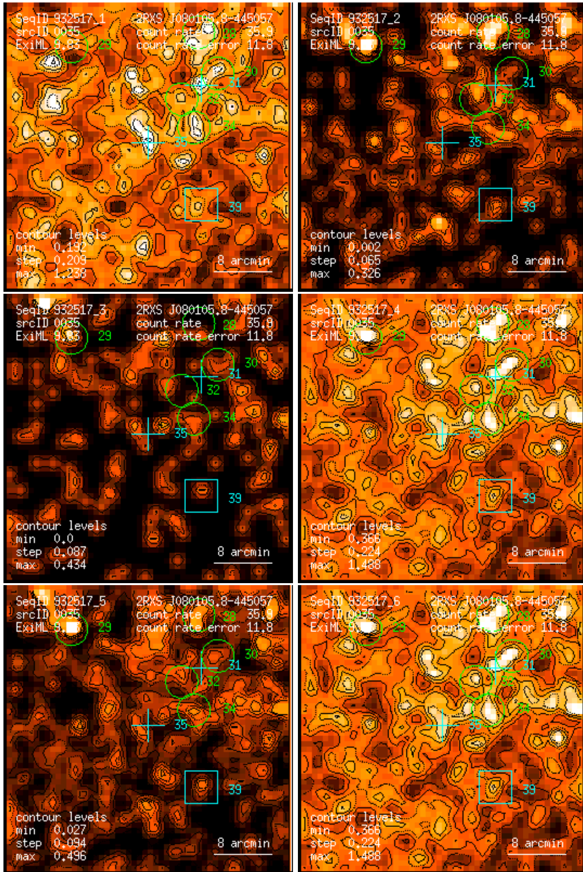
Figure 35: RASS 932517: detection 0035: band rate images, Gaussian filter: (1) PSPC channels 11 – 41, (2) 52 – 90, (3) 91 – 201, (4) 11 – 235, (5) 52 – 201, (6) 11 – 201. Broad band rates in counts/ks. Band rate contour levels in counts/ks/arcmin 2 .
