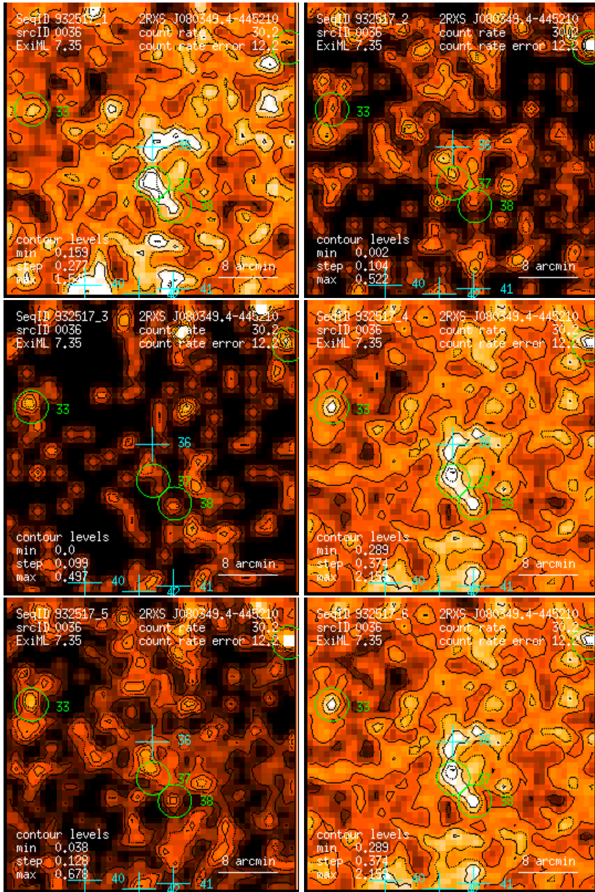
Figure 36: RASS 932517: detection 0036: band rate images, Gaussian filter: (1) PSPC channels 11 – 41, (2) 52 – 90, (3) 91 – 201, (4) 11 – 235, (5) 52 – 201, (6) 11 – 201. Broad band rates in counts/ks. Band rate contour levels in counts/ks/arcmin 2 .
