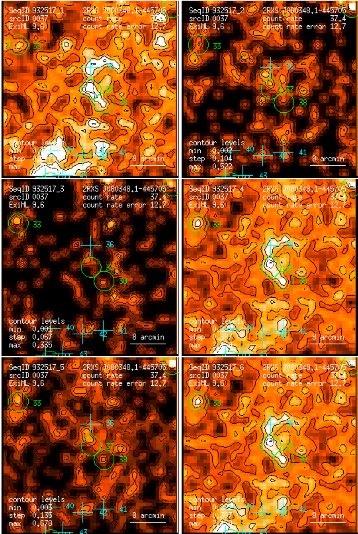
Figure 37: RASS 932517: detection 0037: band rate images, Gaussian filter: (1) PSPC channels 11 – 41, (2) 52 – 90, (3) 91 – 201, (4) 11 – 235, (5) 52 – 201, (6) 11 – 201. Broad band rates in counts/ks. Band rate contour levels in counts/ks/arcmin 2 .
