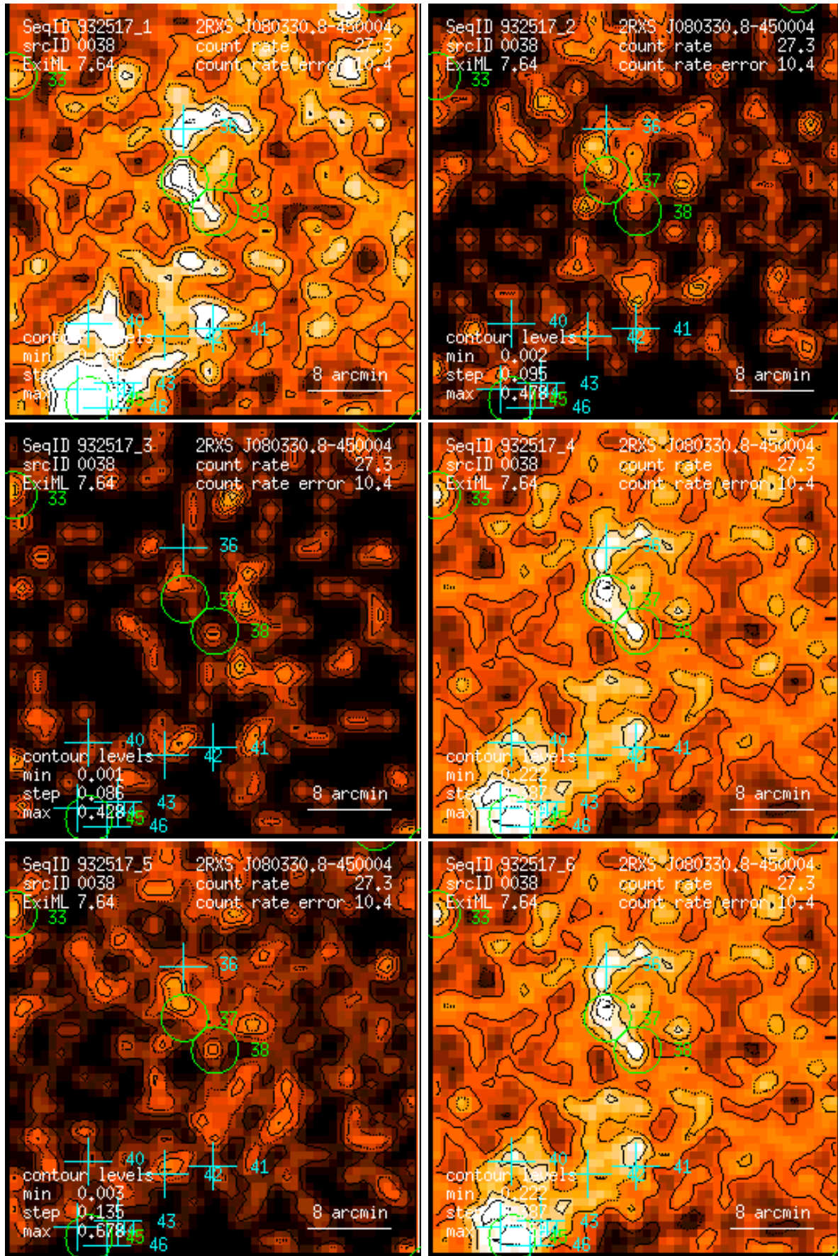
Figure 38: RASS 932517: detection 0038: band rate images, Gaussian filter: (1) PSPC channels 11 – 41, (2) 52 – 90, (3) 91 – 201, (4) 11 – 235, (5) 52 – 201, (6) 11 – 201. Broad band rates in counts/ks. Band rate contour levels in counts/ks/arcmin 2 .
