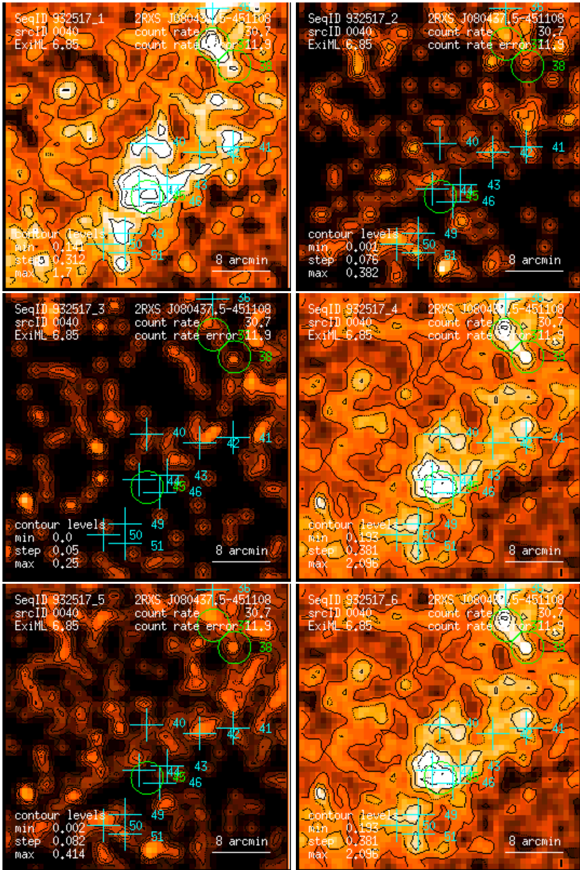
Figure 40: RASS 932517: detection 0040: band rate images, Gaussian filter: (1) PSPC channels 11 – 41, (2) 52 – 90, (3) 91 – 201, (4) 11 – 235, (5) 52 – 201, (6) 11 – 201. Broad band rates in counts/ks. Band rate contour levels in counts/ks/arcmin 2 .
