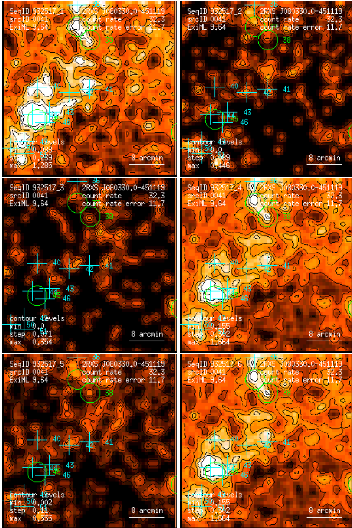
Figure 41: RASS 932517: detection 0041: band rate images, Gaussian filter: (1) PSPC channels 11 – 41, (2) 52 – 90, (3) 91 – 201, (4) 11 – 235, (5) 52 – 201, (6) 11 – 201. Broad band rates in counts/ks. Band rate contour levels in counts/ks/arcmin 2 .
