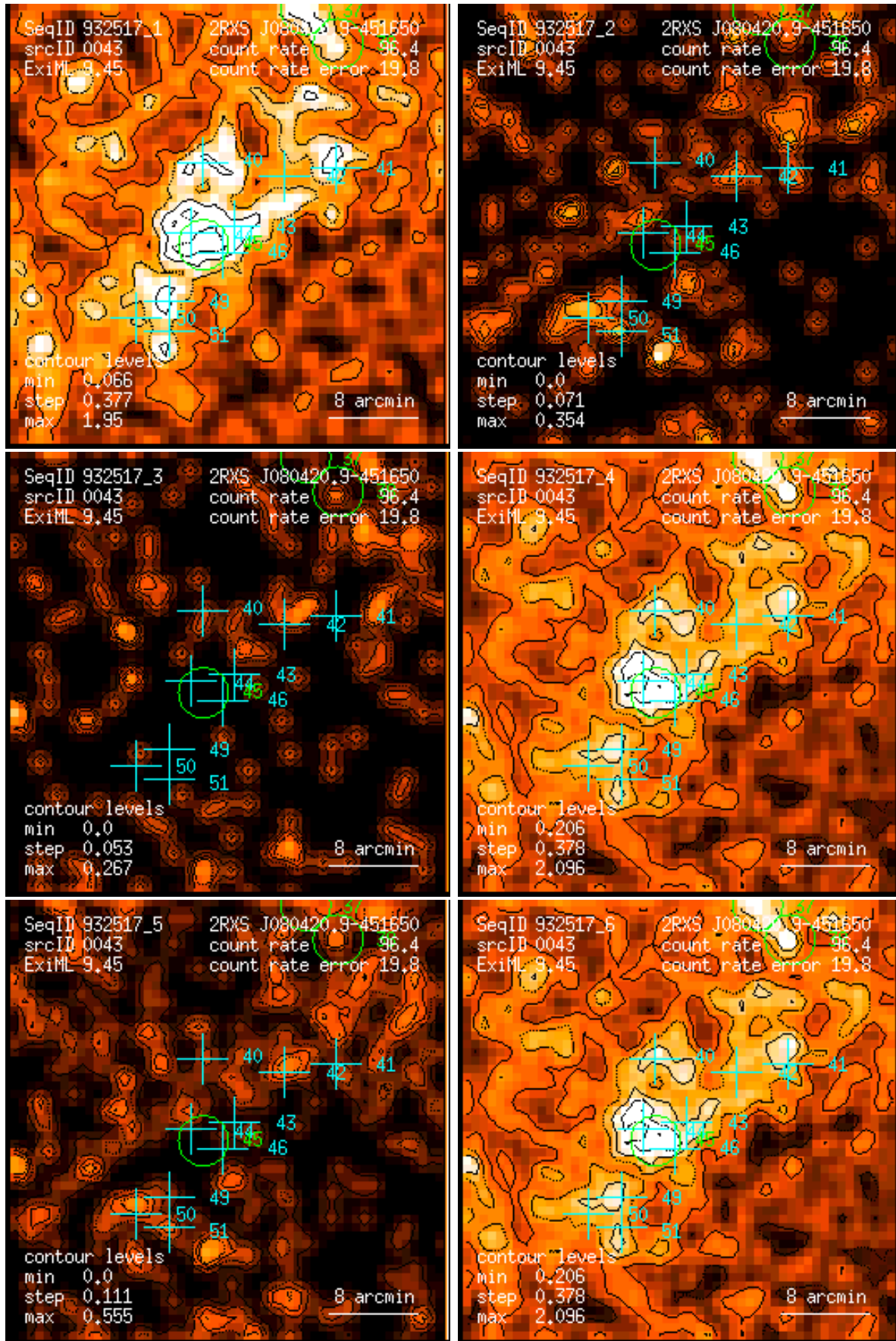
Figure 43: RASS 932517: detection 0043: band rate images, Gaussian filter: (1) PSPC channels 11 – 41, (2) 52 – 90, (3) 91 – 201, (4) 11 – 235, (5) 52 – 201, (6) 11 – 201. Broad band rates in counts/ks. Band rate contour levels in counts/ks/arcmin 2 .
