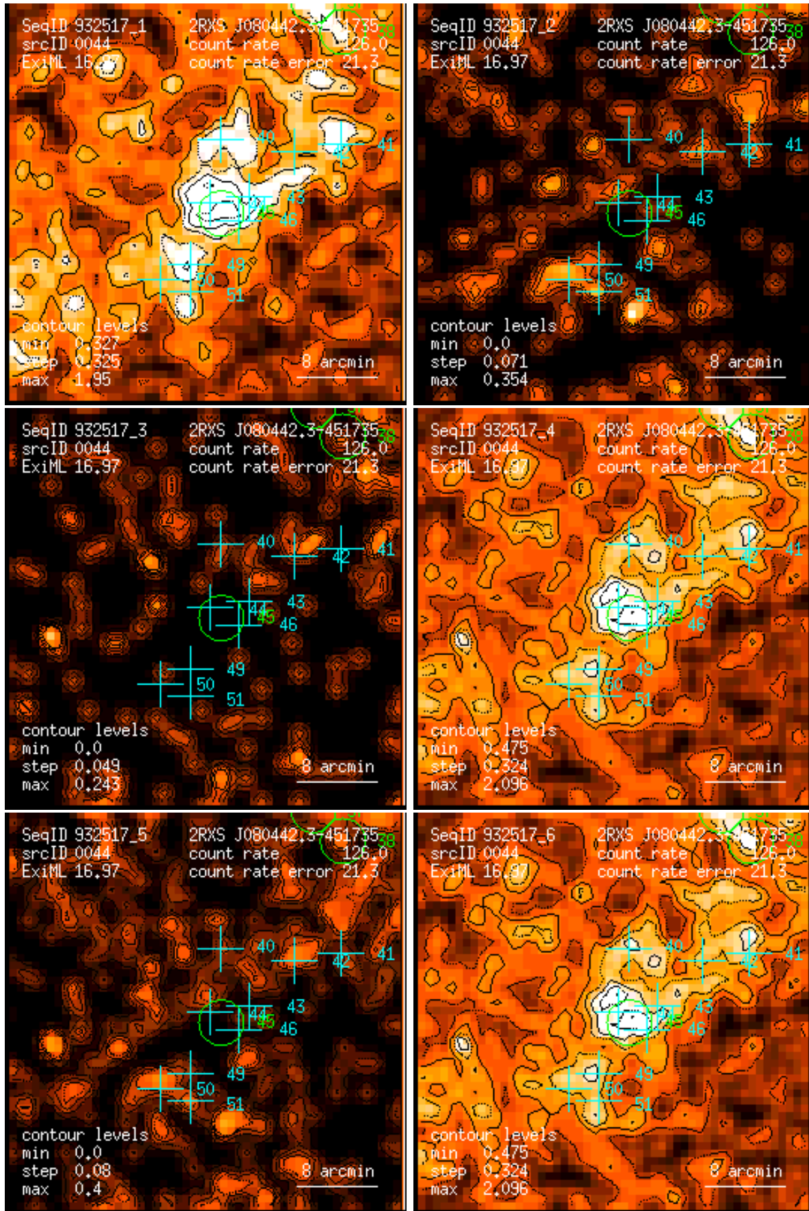
Figure 44: RASS 932517: detection 0044: band rate images, Gaussian filter: (1) PSPC channels 11 – 41, (2) 52 – 90, (3) 91 – 201, (4) 11 – 235, (5) 52 – 201, (6) 11 – 201. Broad band rates in counts/ks. Band rate contour levels in counts/ks/arcmin 2 .
