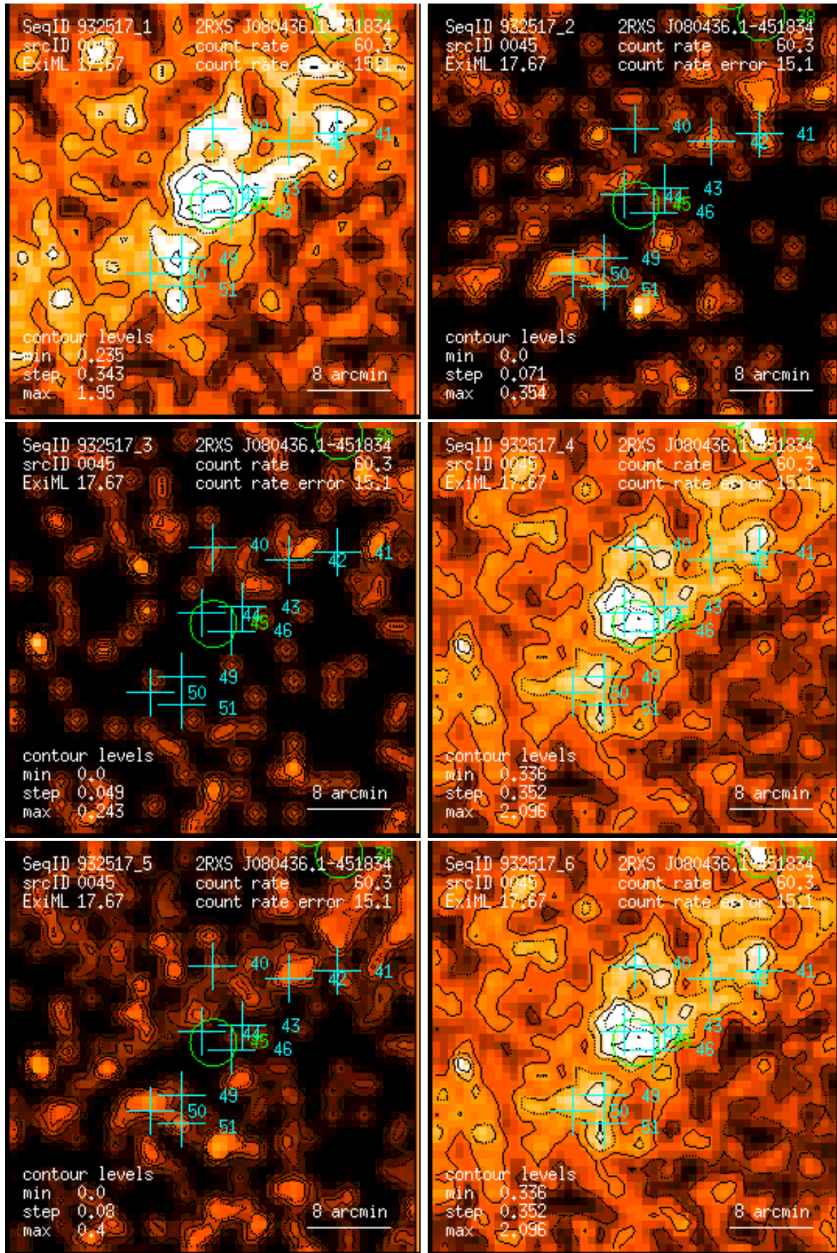
Figure 45: RASS 932517: detection 0045: band rate images, Gaussian filter: (1) PSPC channels 11 – 41, (2) 52 – 90, (3) 91 – 201, (4) 11 – 235, (5) 52 – 201, (6) 11 – 201. Broad band rates in counts/ks. Band rate contour levels in counts/ks/arcmin 2 .
