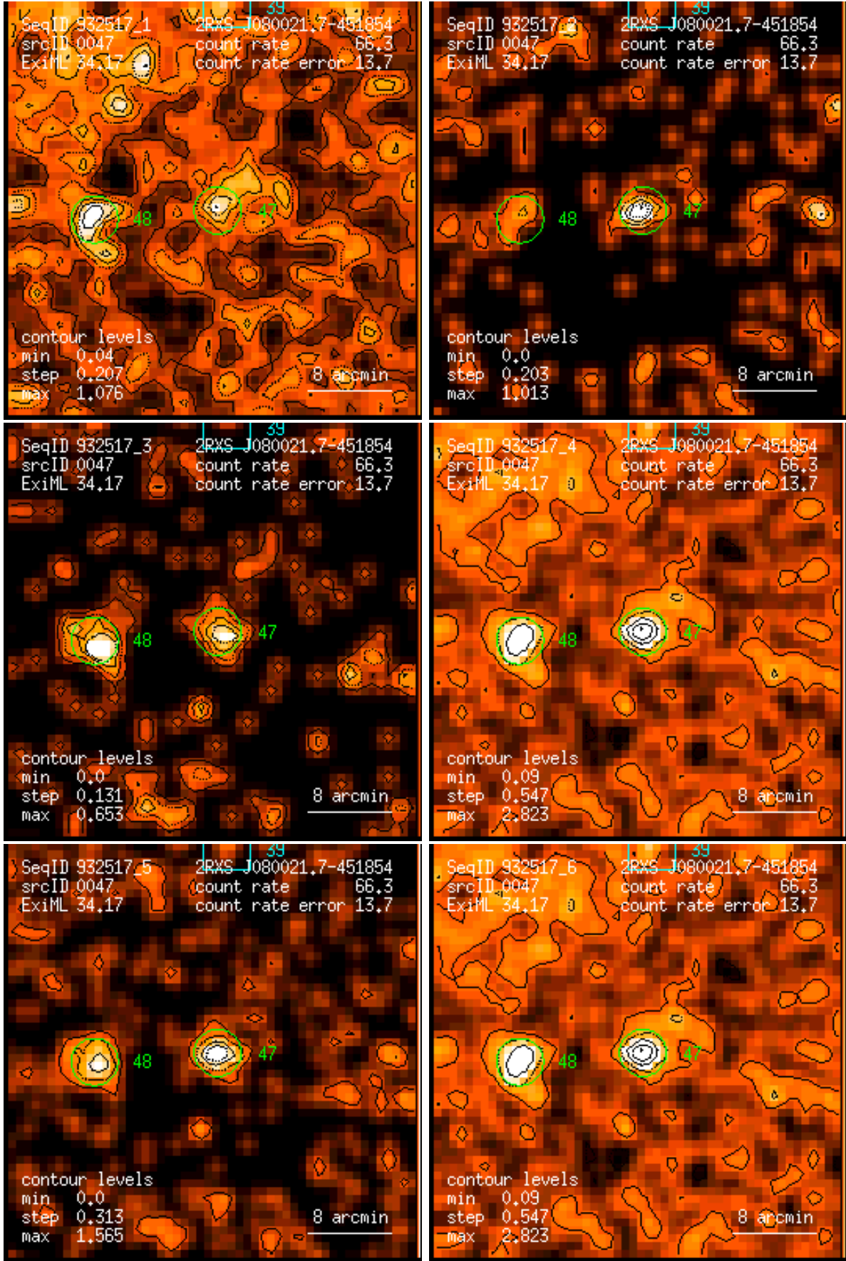
Figure 47: RASS 932517: detection 0047: band rate images, Gaussian filter: (1) PSPC channels 11 – 41, (2) 52 – 90, (3) 91 – 201, (4) 11 – 235, (5) 52 – 201, (6) 11 – 201. Broad band rates in counts/ks. Band rate contour levels in counts/ks/arcmin 2 .
